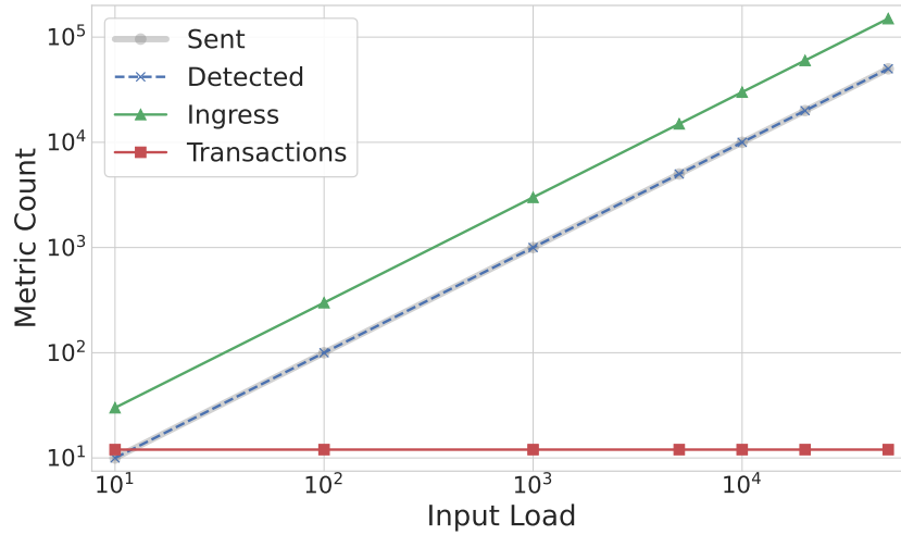
Figure 6.4: Evolution of SPS processing metrics under increasing input load N , measured in attacks sent from the attacker machine: sent payloads, alerts detected by the most virtuous IDS, total ingress traffic received at the blockchain-facing nodes, and finalized blockchain transactions. Both axes are shown in logarithmic scale. Results are reported for the CometBFT configuration.
