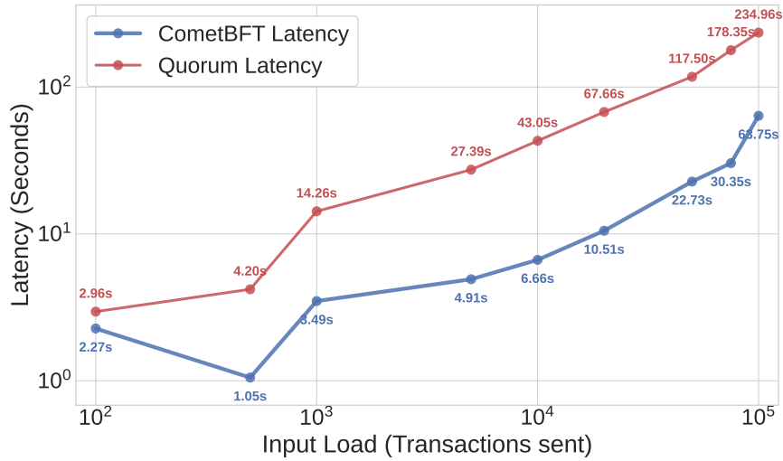
Figure 7.2: Burst completion latency as a function of the input load, on logarithmic axes, for the two blockchain configurations. Annotated values report the wall-clock time in seconds required to drain each burst.
