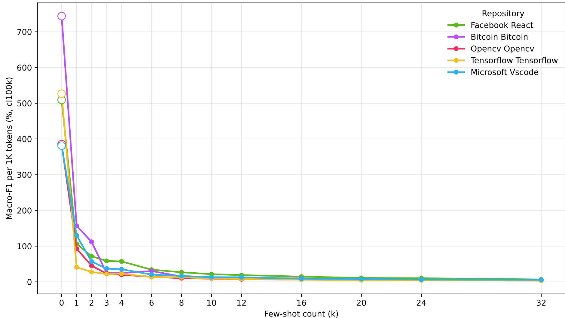
Mistral-7B-Instruct-v0.3
