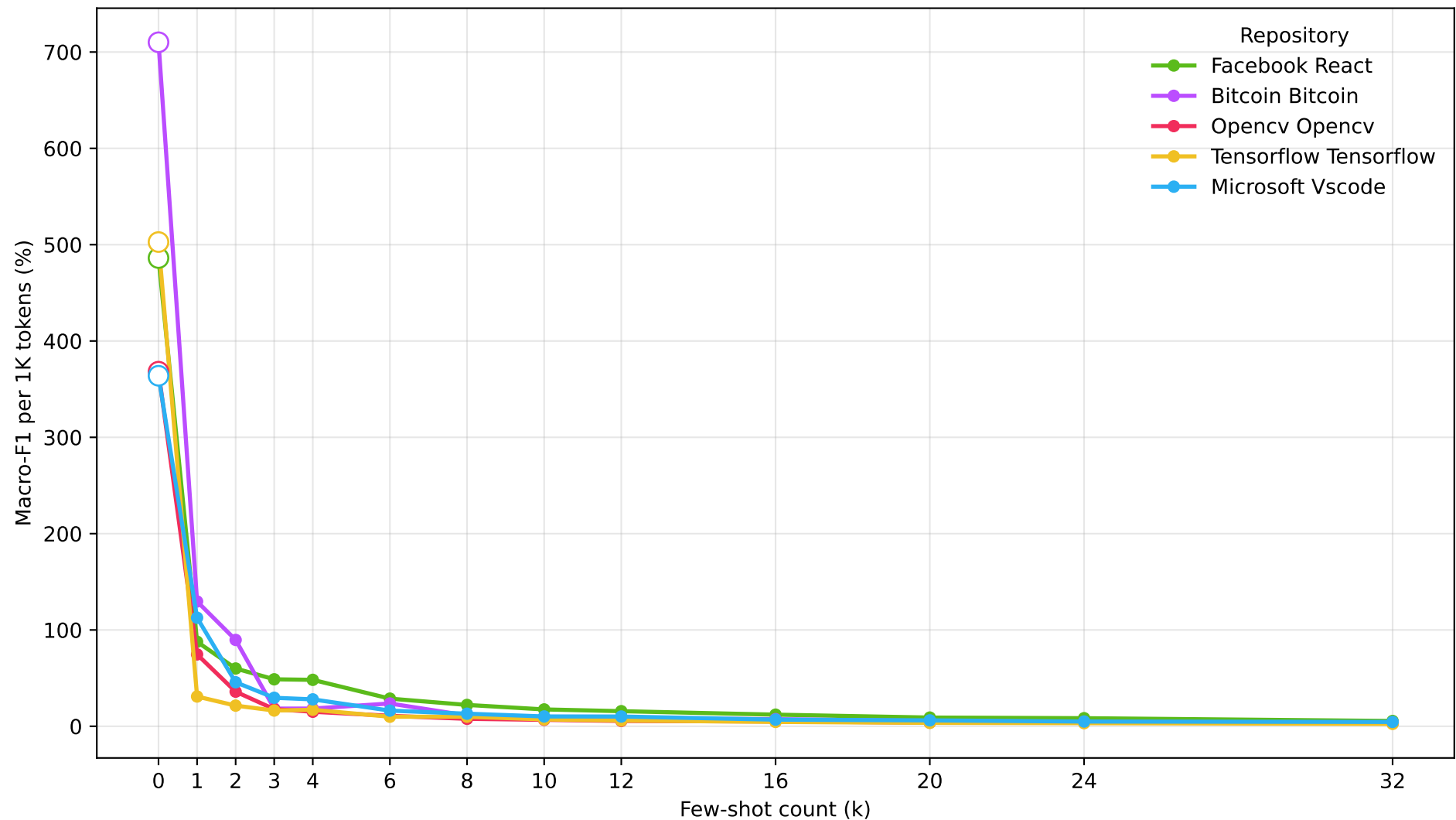
Mistral-7B-Instruct-v0.3
