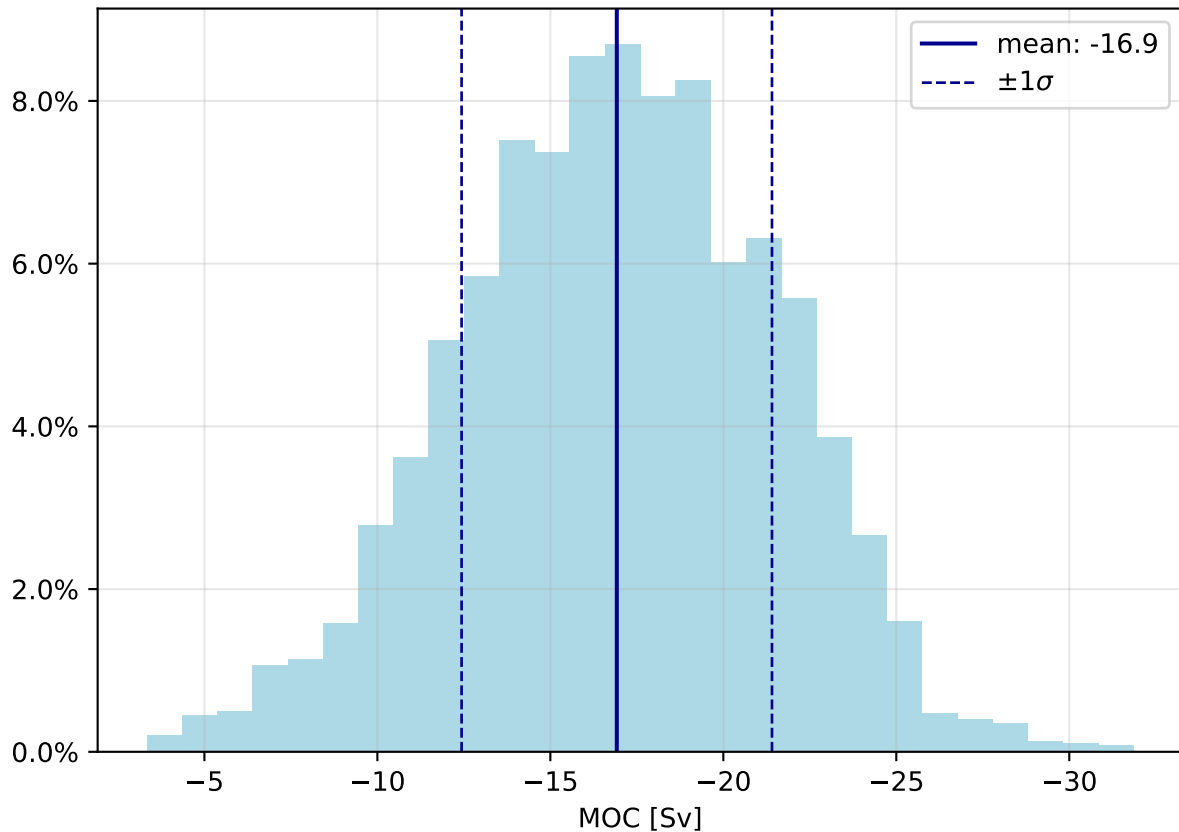
MOVE 16°N - NADW Transport Distribution
