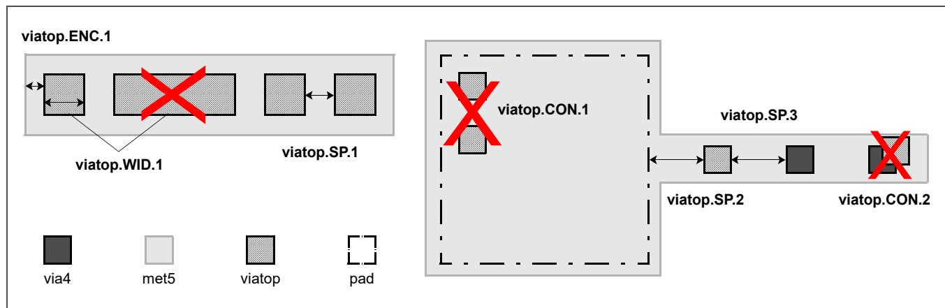
Figure 3-14. Topside Via Layout
