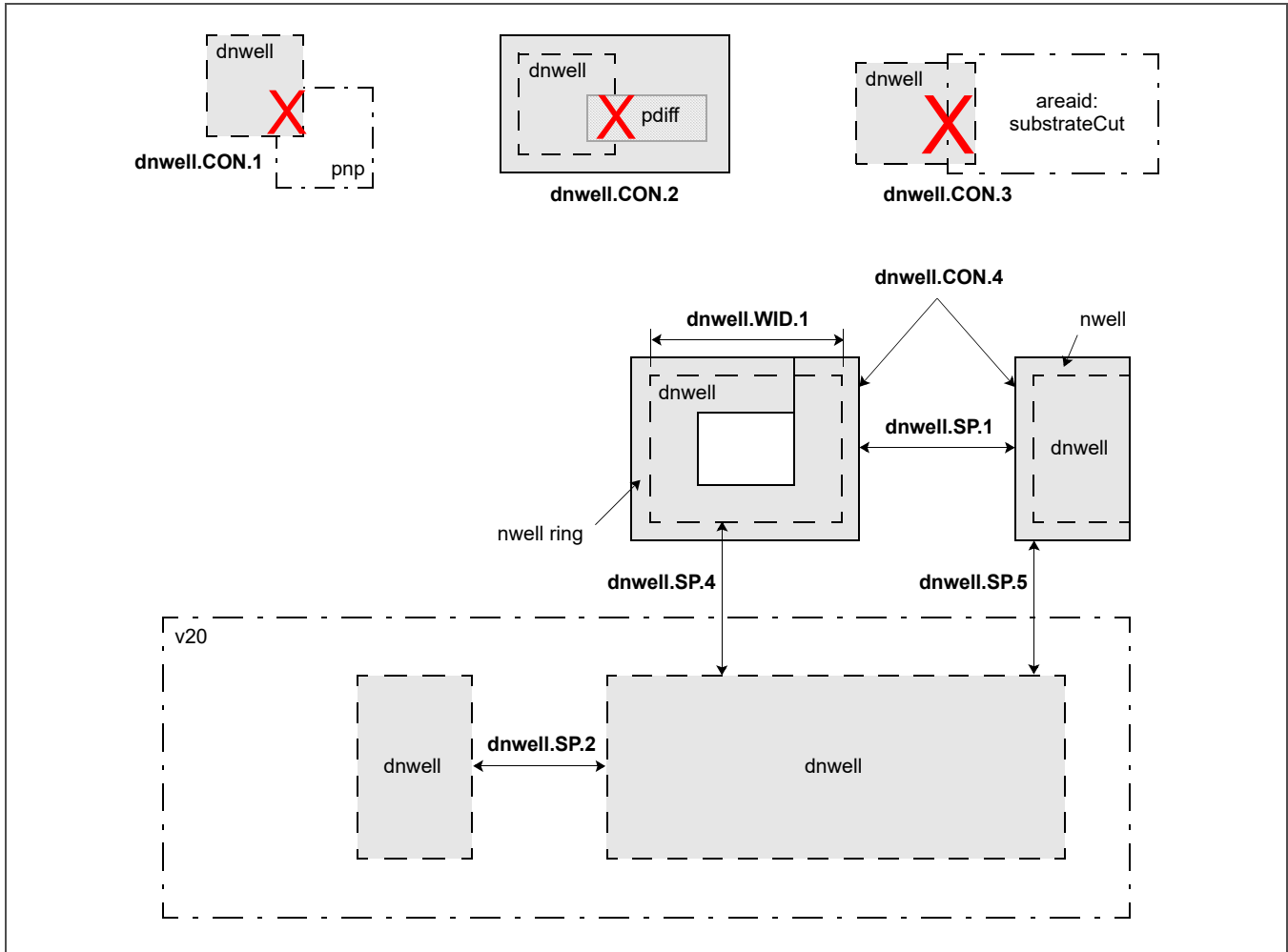
Figure 3-1. Deep N-Well Layout
