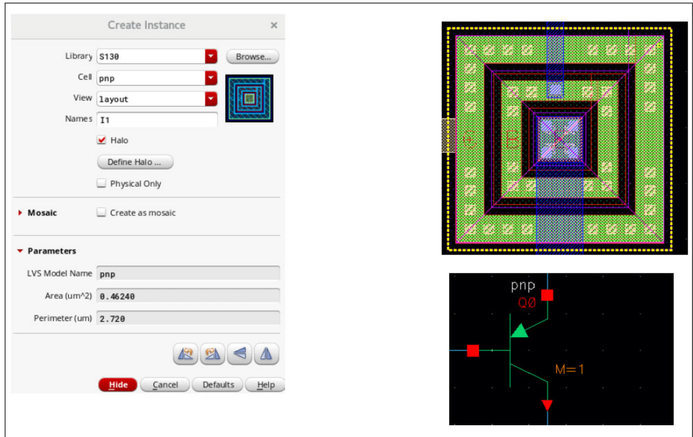
Figure 3-25. PNP Cell Layout
