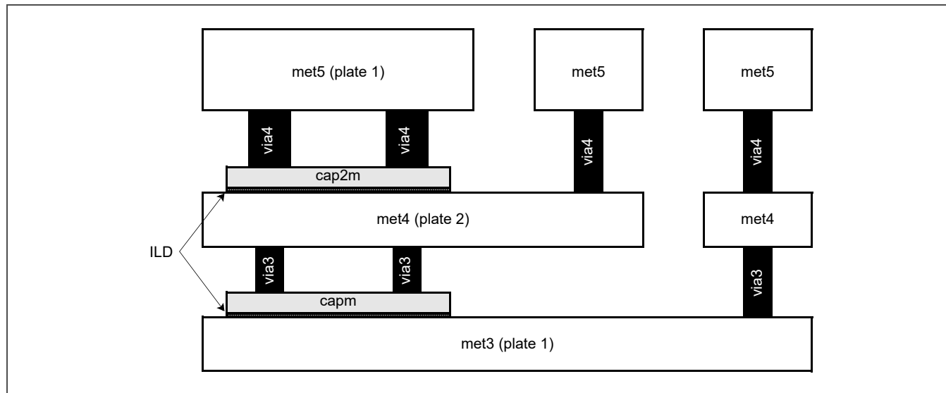
Figure 3-26. Stacked MIM Capacitor Cross Section
