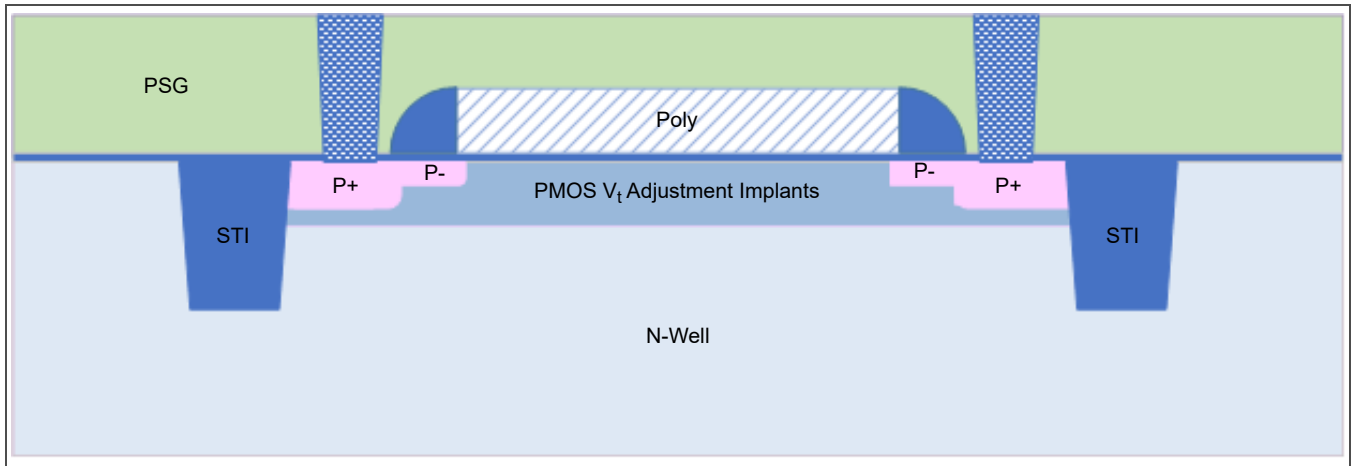
Figure 3-15. High- V_t PFET Cross Section
