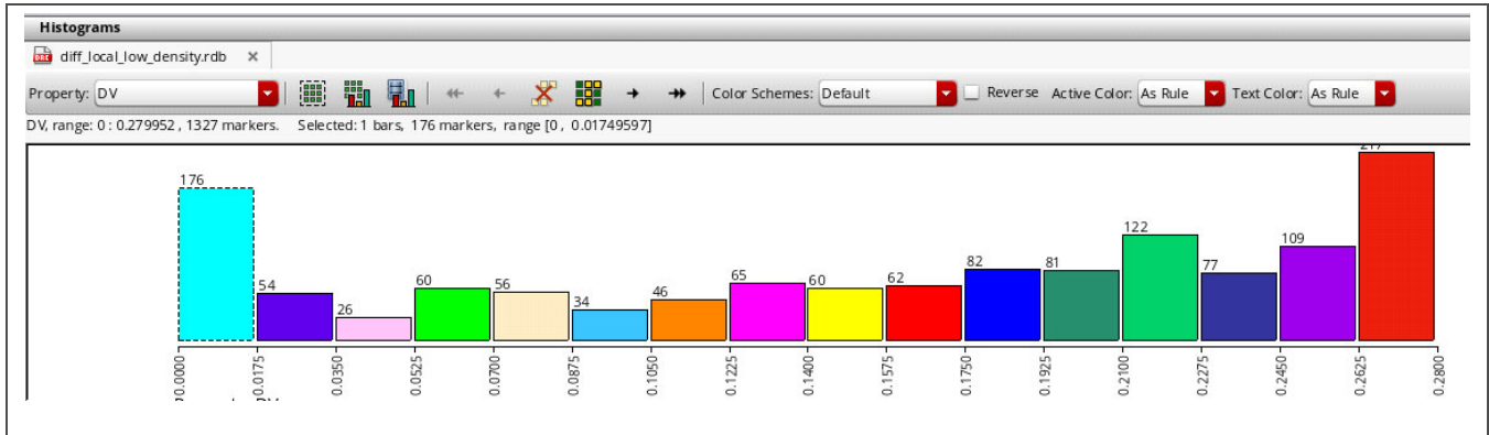
Figure A-22. PVS Low Diffusion Local Density Histogram Example 2
