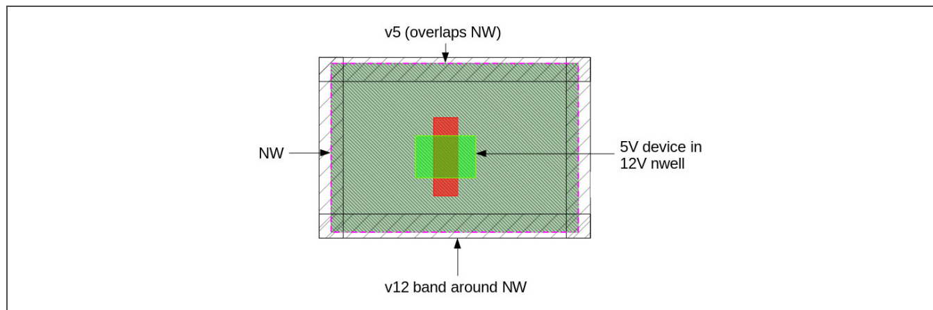
Figure 2-4. Example of a High-Voltage Marker Layer Exception
