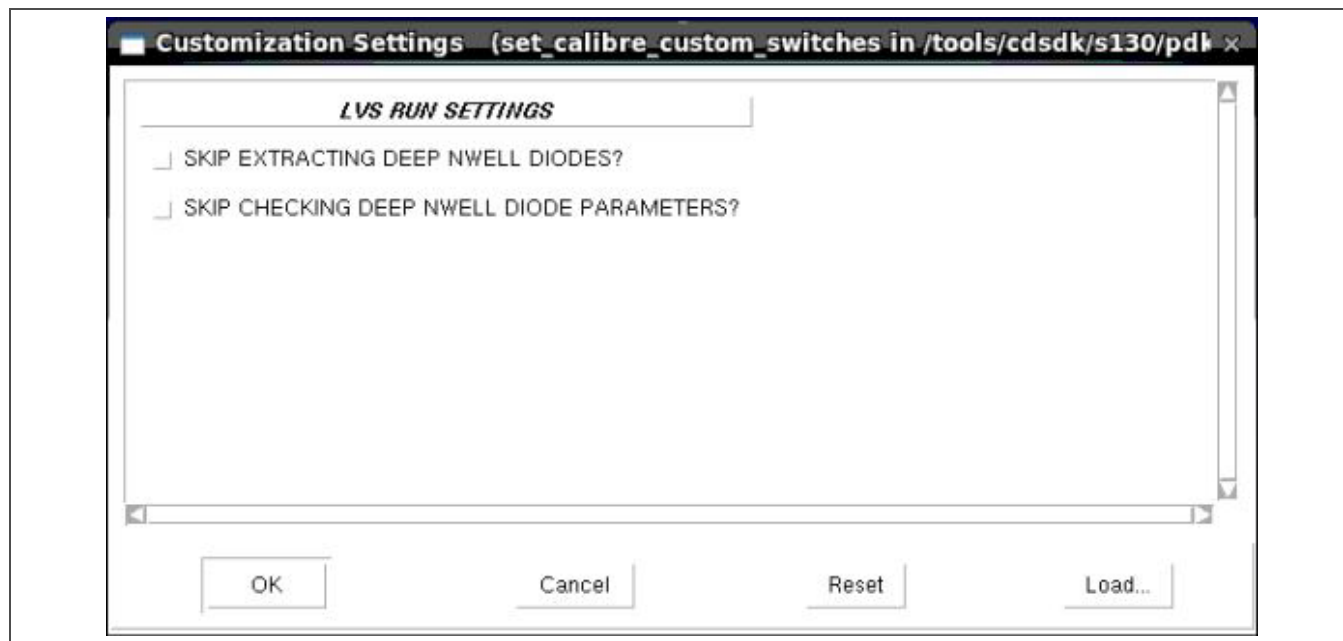
Figure 5-2. Calibre LVS Customization Form
