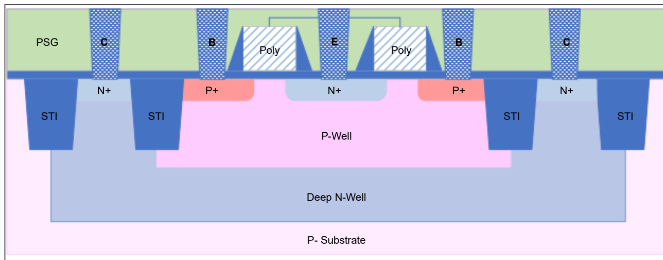
Figure 3-22. 5\text{ V } 1 \times 1 NPN Transistor Cross Section
