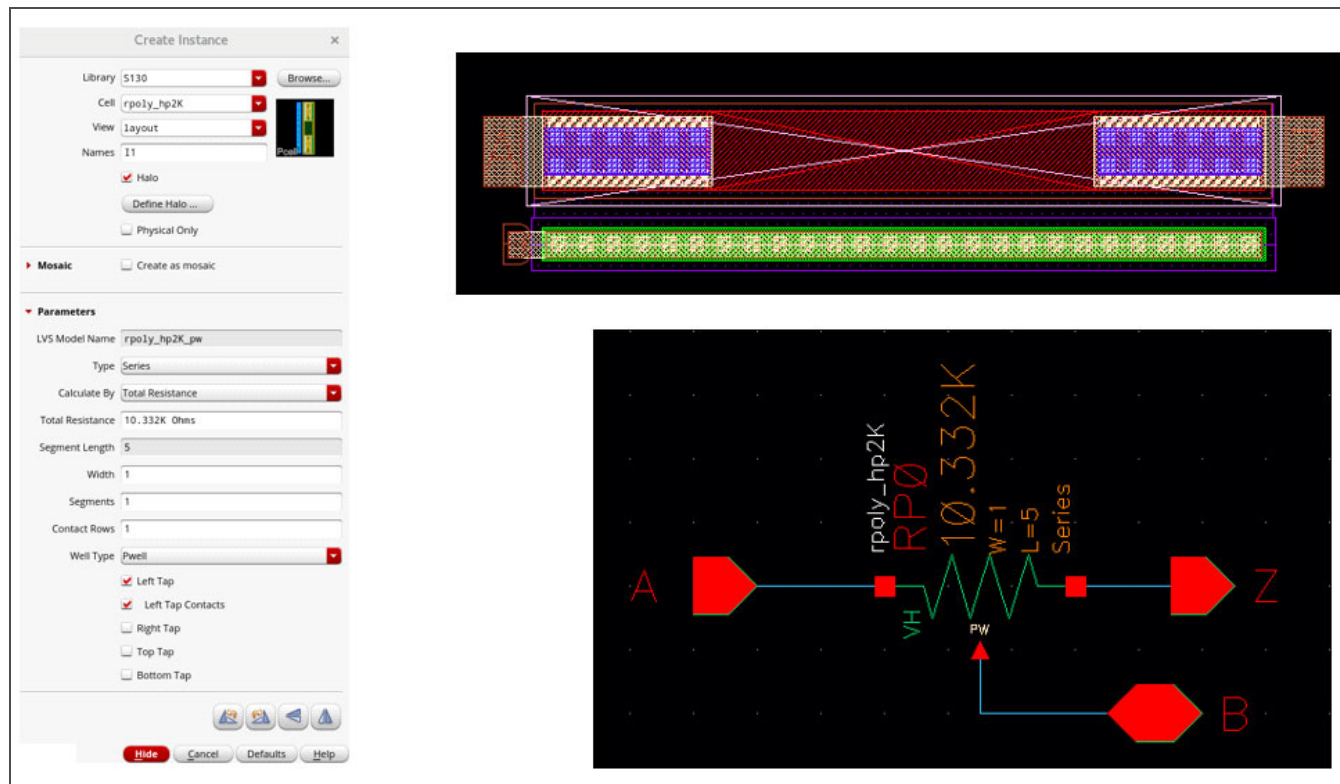
Figure 3-38. High Sheet Rho Poly Resistor Pcell Layout
