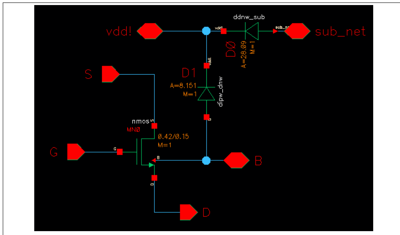
Figure 2-9. Schematic Example of an N+ Transistor in an Isolated P+ Substrate
