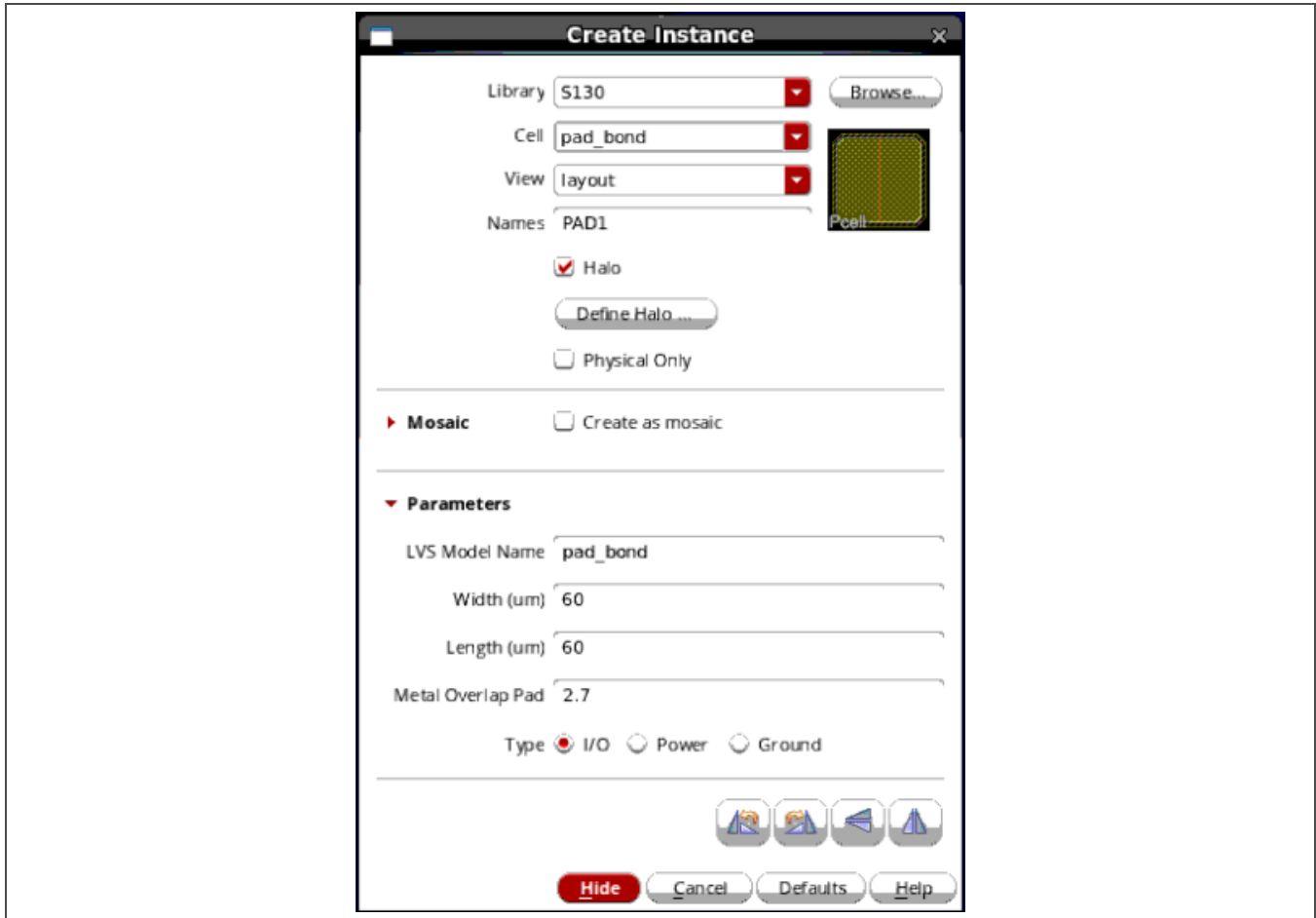
Figure 2-5. Pad Marker Selection in Bond-Pad Pcell Create Instance Form
