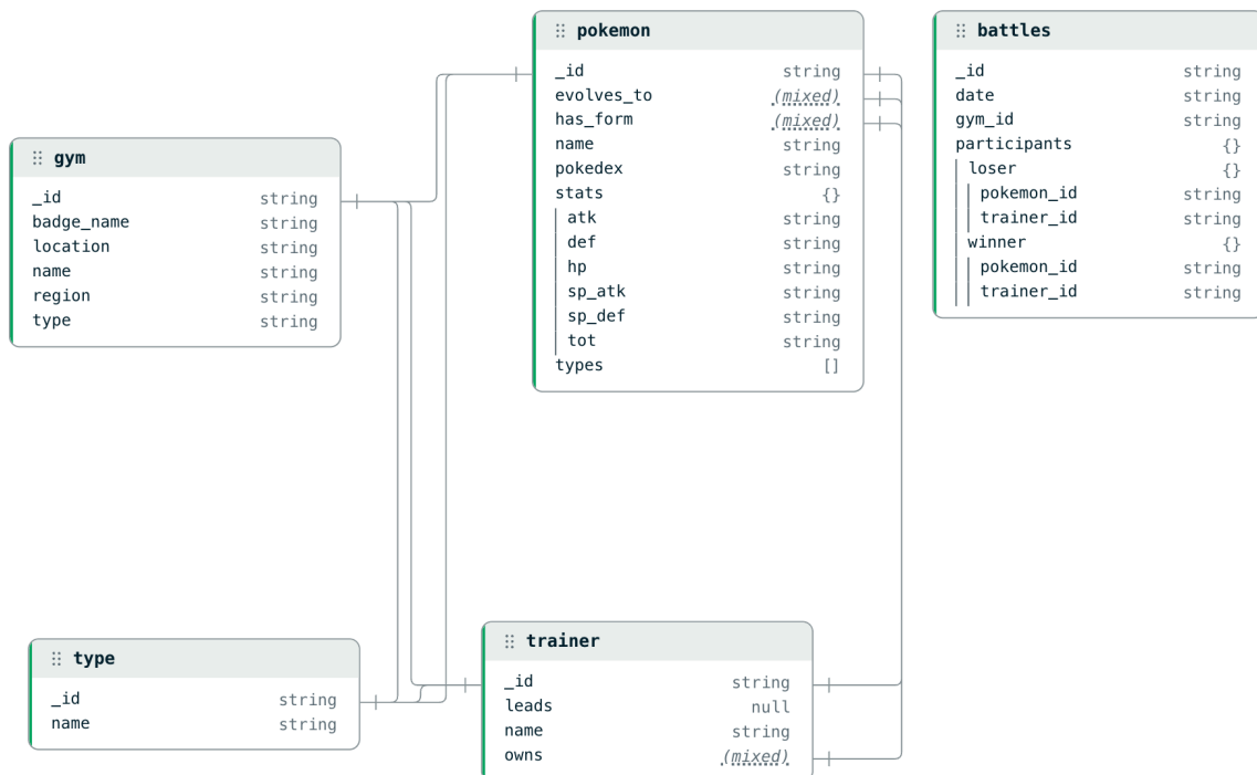
Figure 3: MongoDB structure
