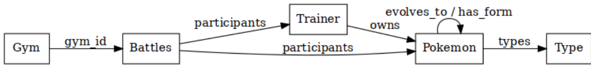
Figure 1: MongoDB schema relationships in brief
