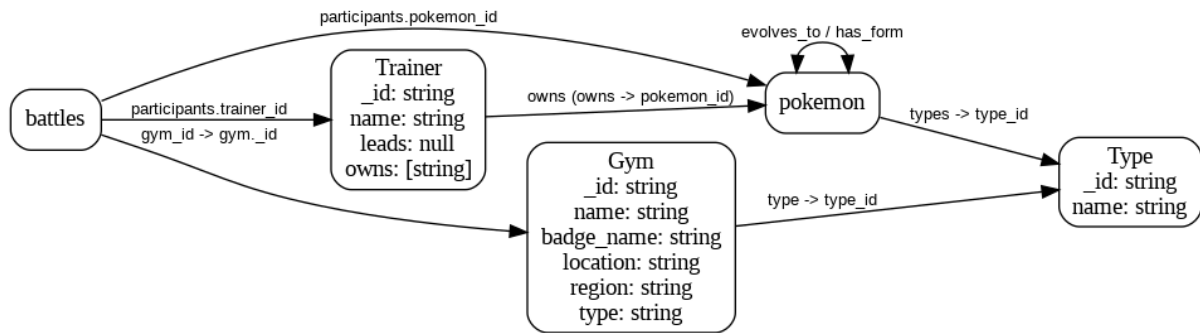
Figure 2: MongoDB full schema relationships
