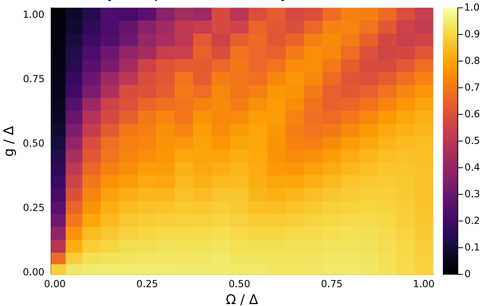
Fidelity, step 1, non-unitary, with correction
