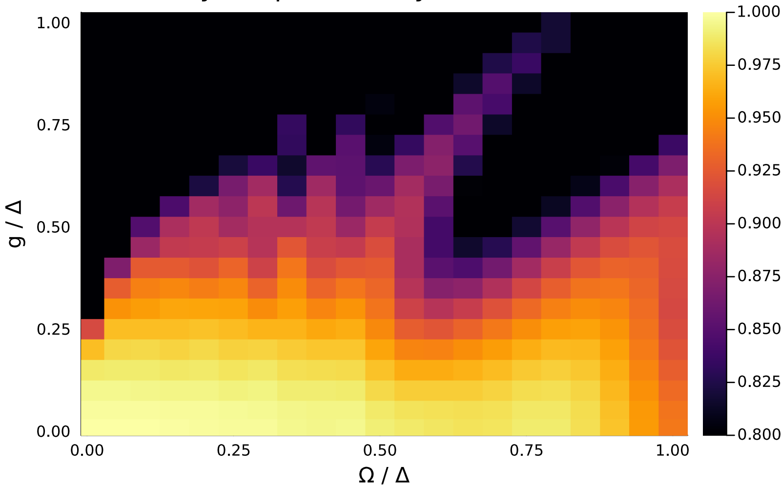
Fidelity, step 1, unitary, with correction
