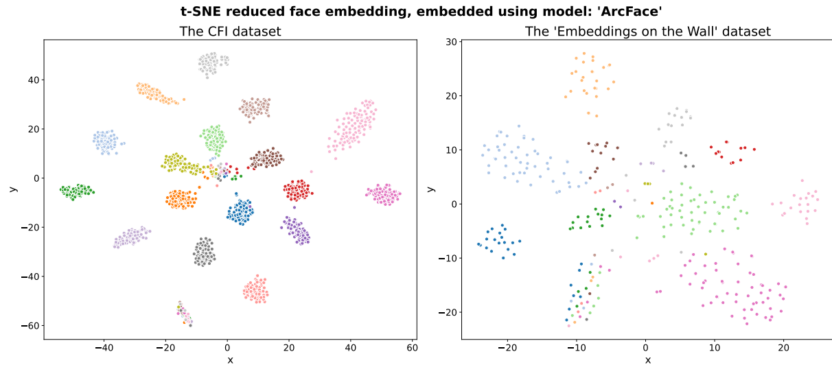
Figure 18: Actual cluster of all faces in both the CFI dataset (left) and the Embedding on the Wall dataset (right) embedded using the ArcFace model. Each color defines a unique person.
