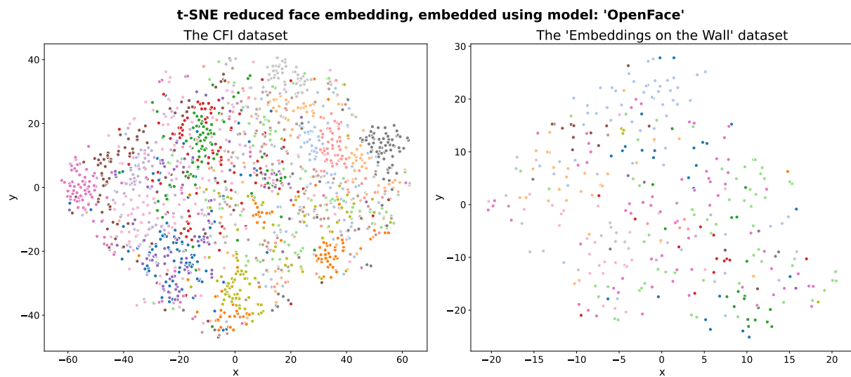
Figure 23: Actual cluster of all faces in both the CFI dataset (left) and the Embedding on the Wall dataset (right) embedded using the OpenFace model. Each color defines a unique person.
