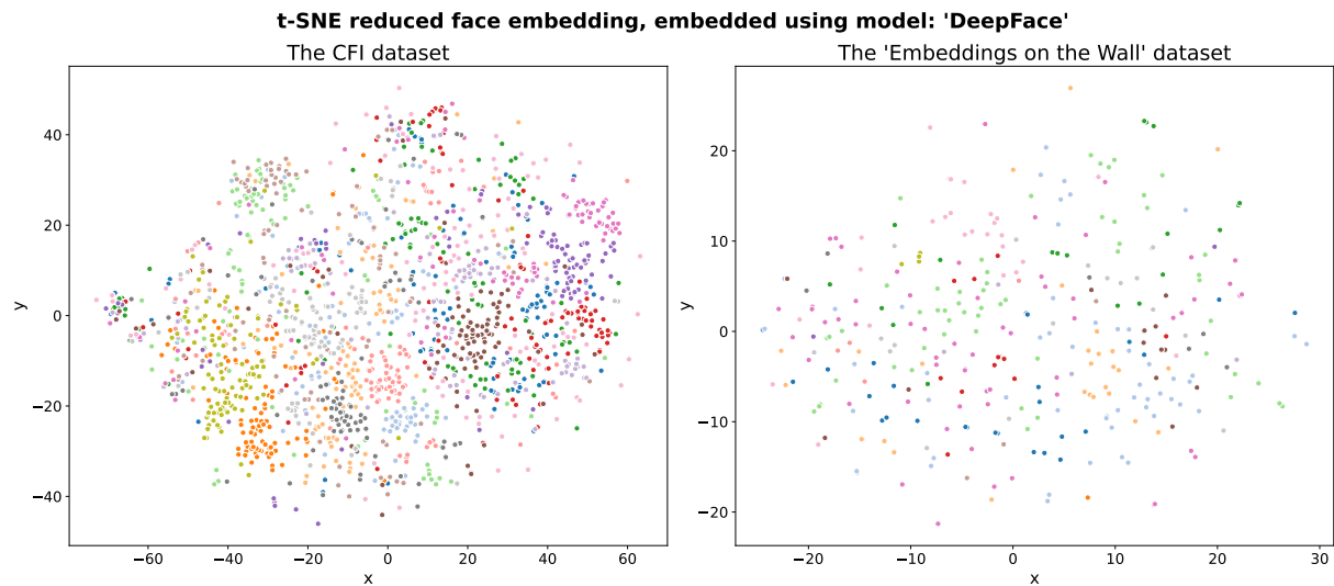
Figure 19: Actual cluster of all faces in both the CFI dataset (left) and the Embedding on the Wall dataset (right) embedded using the DeepFace model. Each color defines a unique person.
