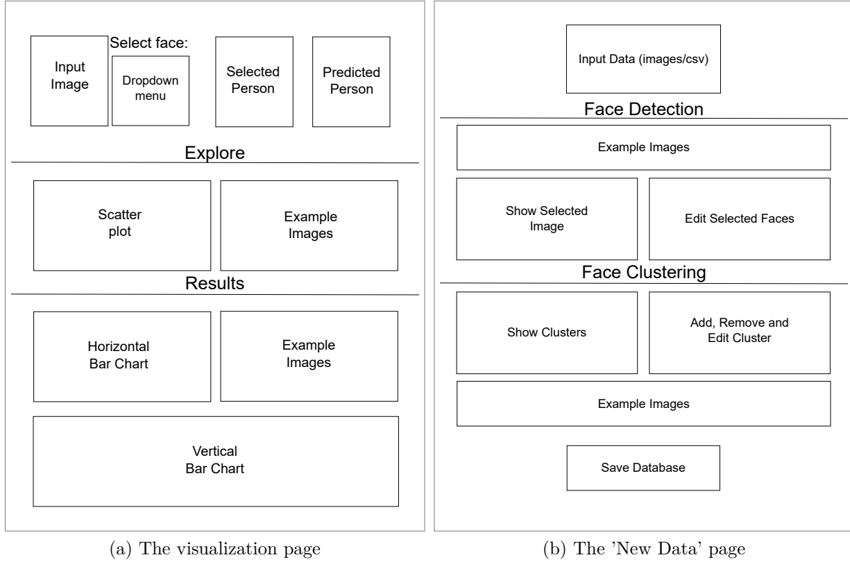
Figure 7: Sketch of the interactive visualization, consisting of two pages.
