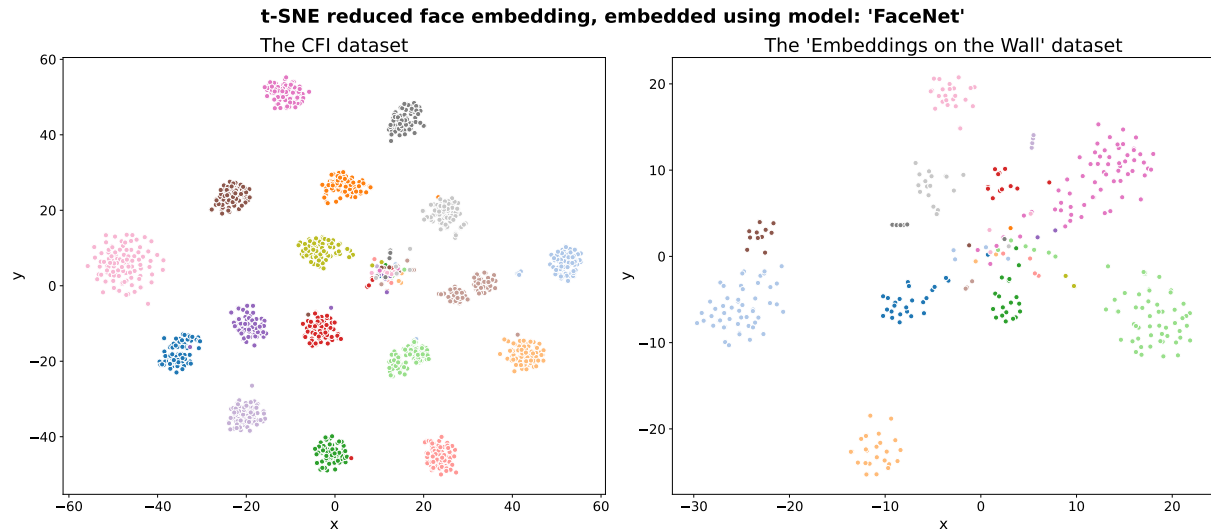
Figure 22: Actual cluster of all faces in both the CFI dataset (left) and the Embedding on the Wall dataset (right) embedded using the FaceNet model. Each color defines a unique person.
