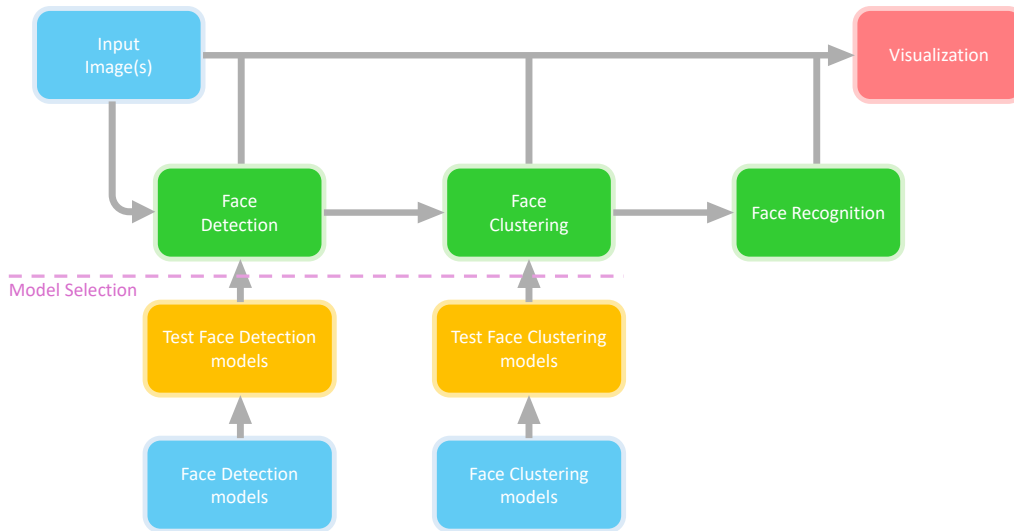
Figure 5: Flowchart displaying the approach of the main steps of the methodology.
