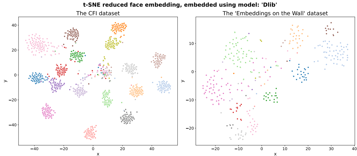
Figure 20: Actual cluster of all faces in both the CFI dataset (left) and the Embedding on the Wall dataset (right) embedded using the Dlib model. Each color defines a unique person.
