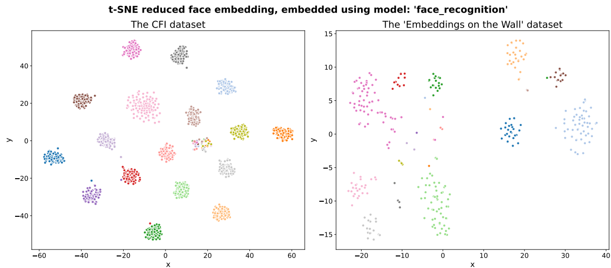
Figure 21: Actual cluster of all faces in both the CFI dataset (left) and the Embedding on the Wall dataset (right) embedded using the face_recognition model. Each color defines a unique person.
