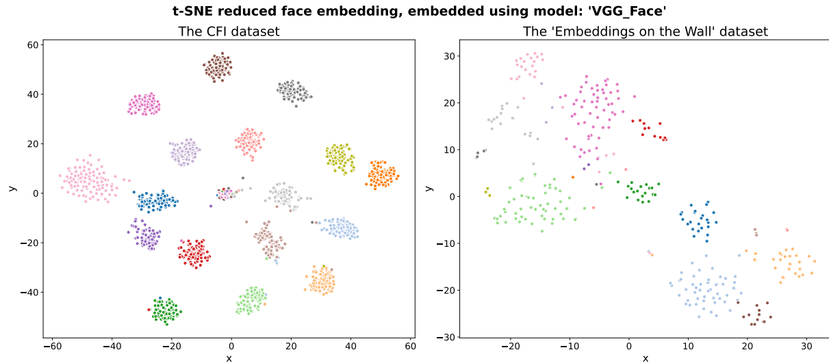
Figure 24: Actual cluster of all faces in both the CFI dataset (left) and the Embedding on the Wall dataset (right) embedded using the VGG_Face model. Each color defines a unique person.
