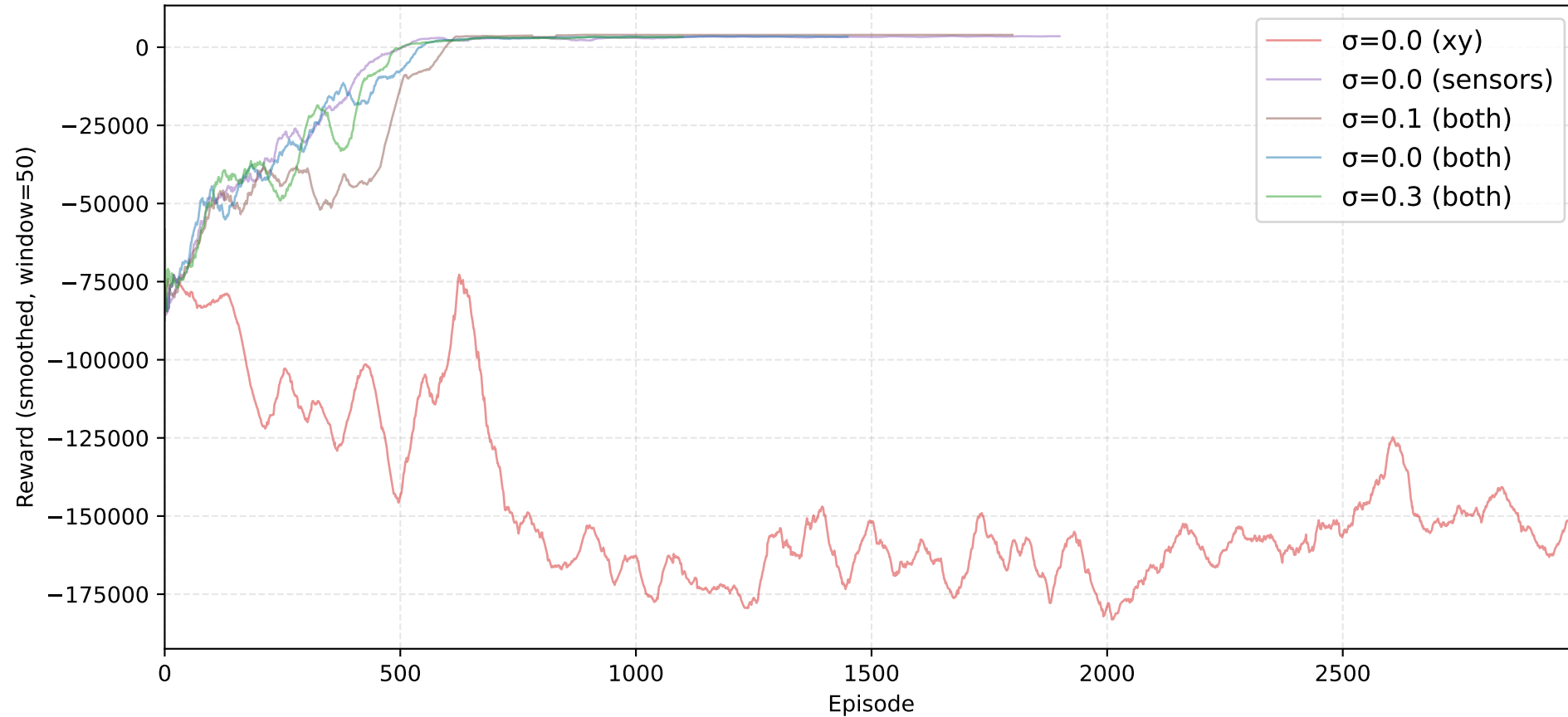
DQN convergence by obs_mode and sigma
