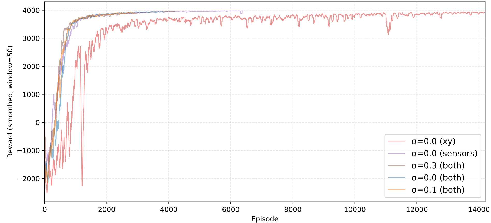
PPO convergence by obs_mode and sigma
