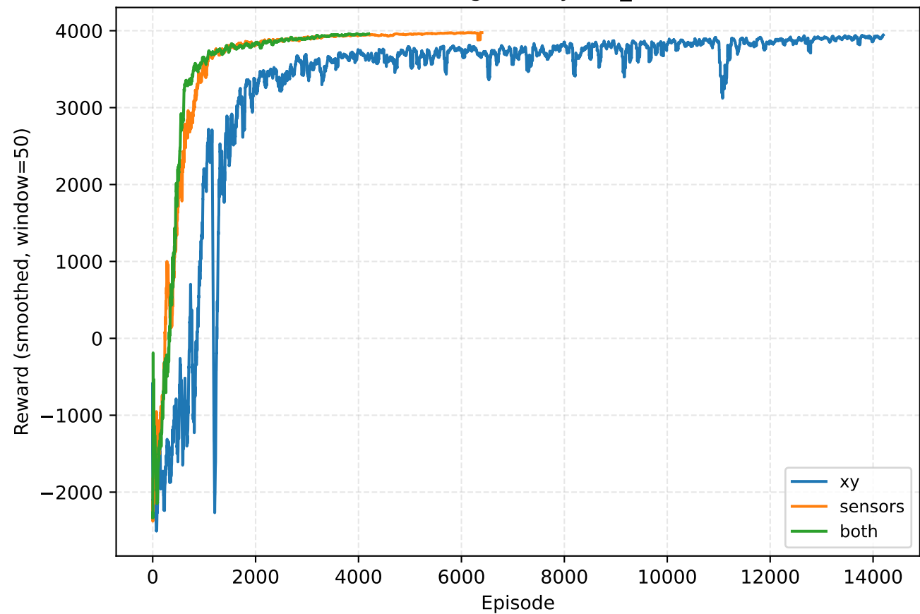
PPO convergence by obs_mode
