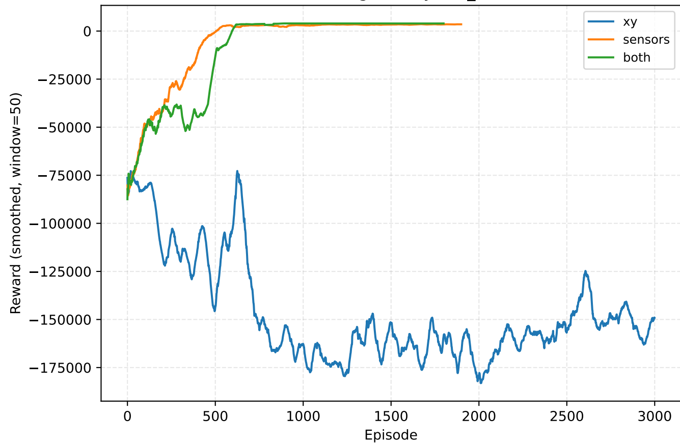
DQN convergence by obs_mode
