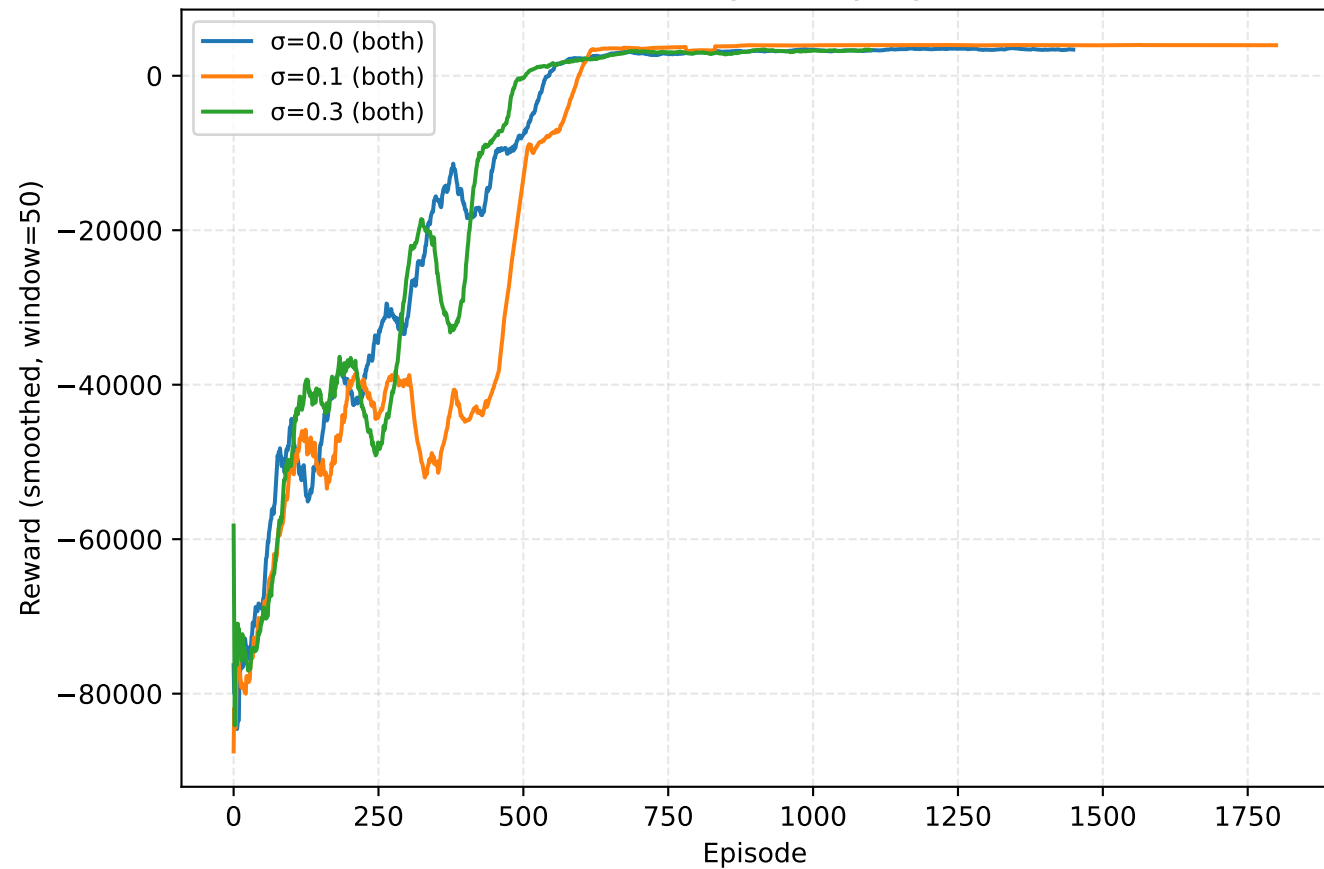
DQN convergence by sigma
