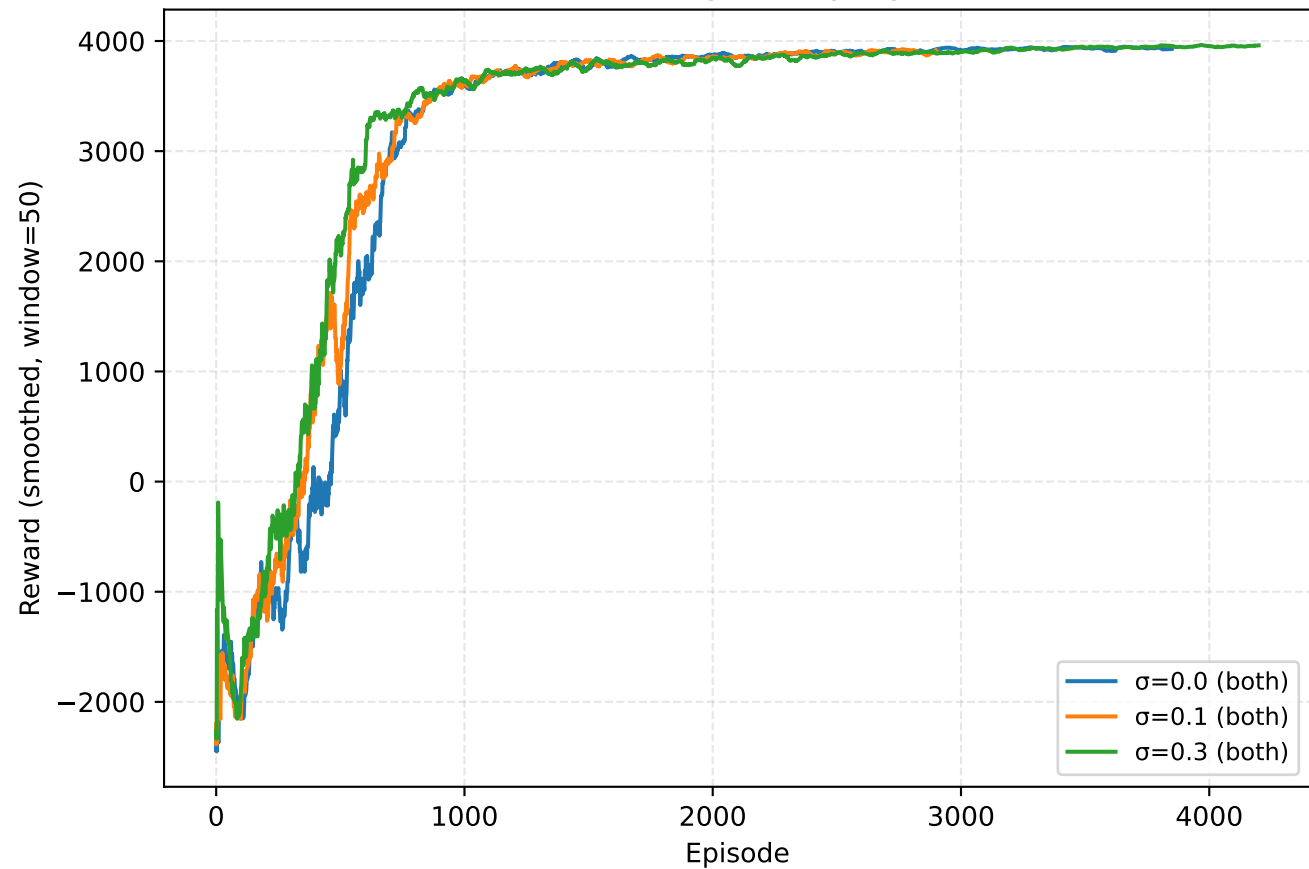
PPO convergence by sigma
