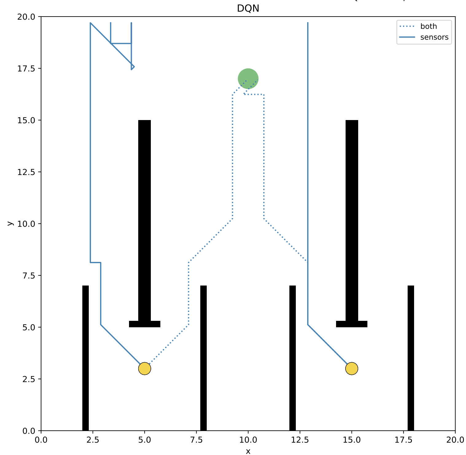
DQN vs PPO, sensors vs both (symmetric_2_space)
