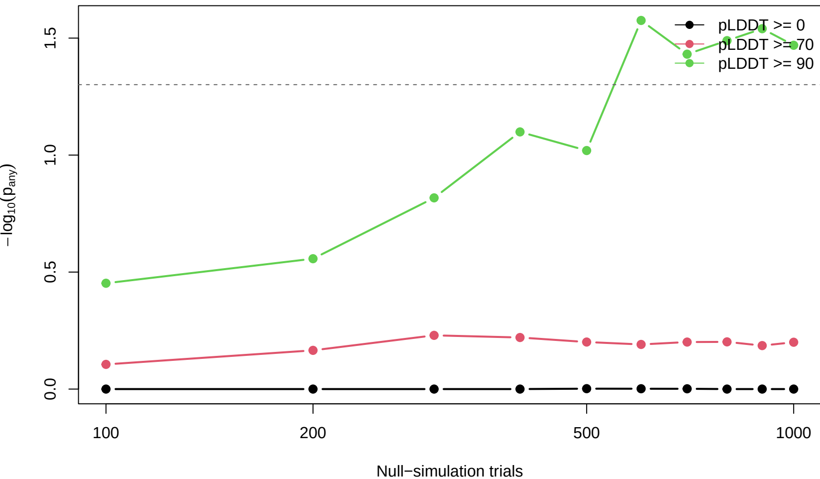
EZH2 cluster_0100 empirical p-value
