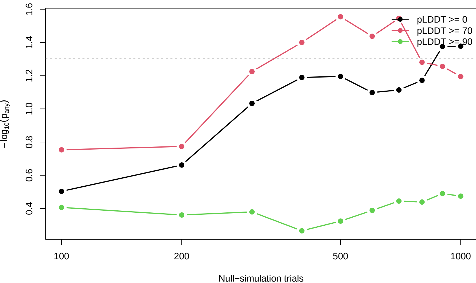
LEF1 cluster_0006 empirical p-value
