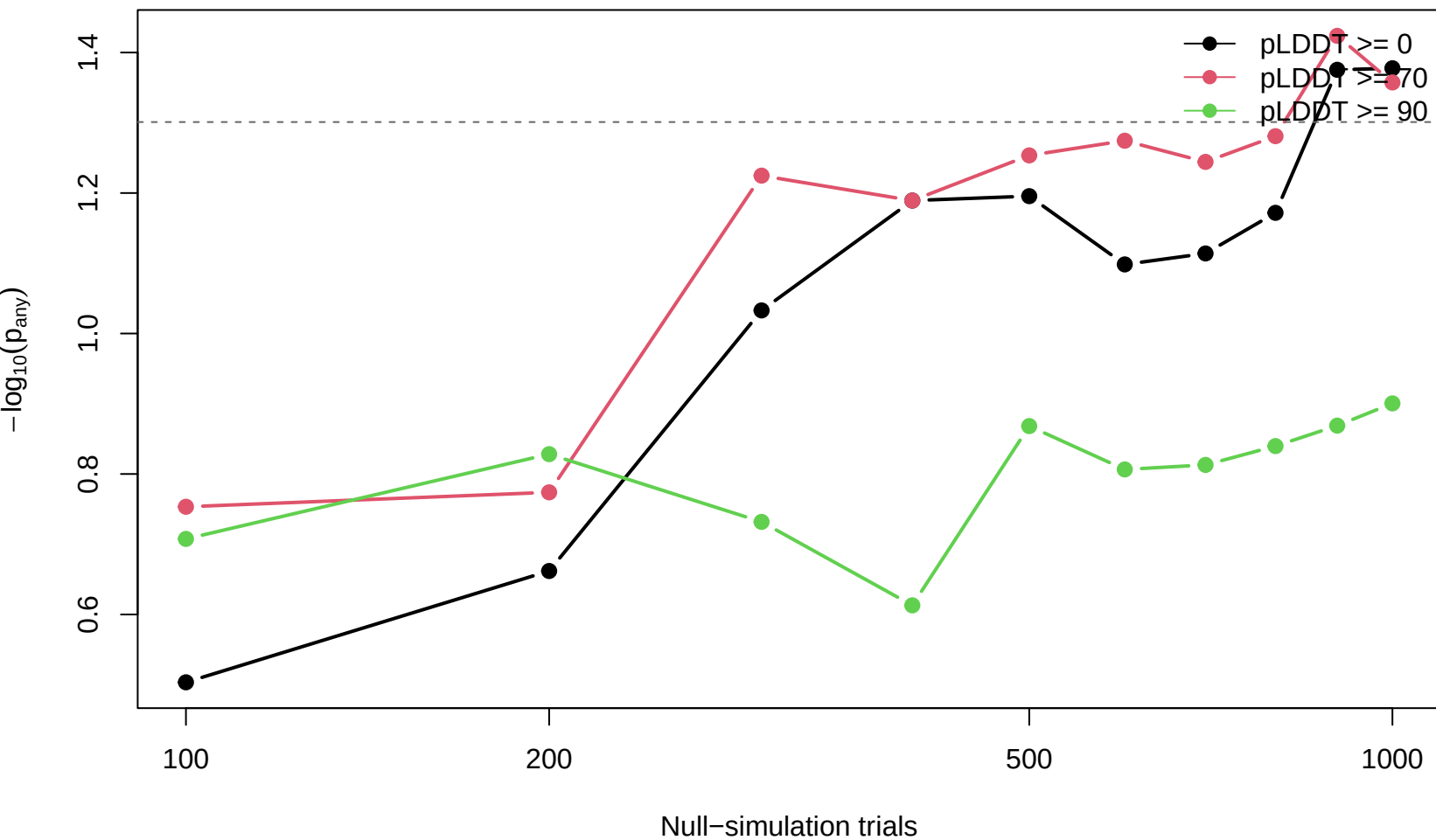
LEF1 cluster_0008 empirical p-value
