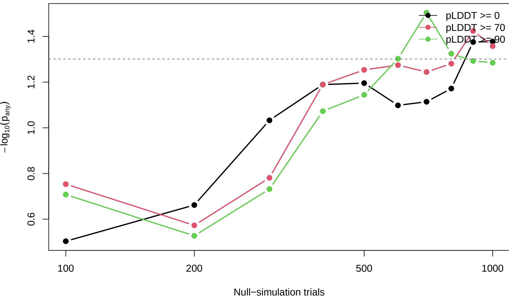
LEF1 cluster_0001 empirical p-value
