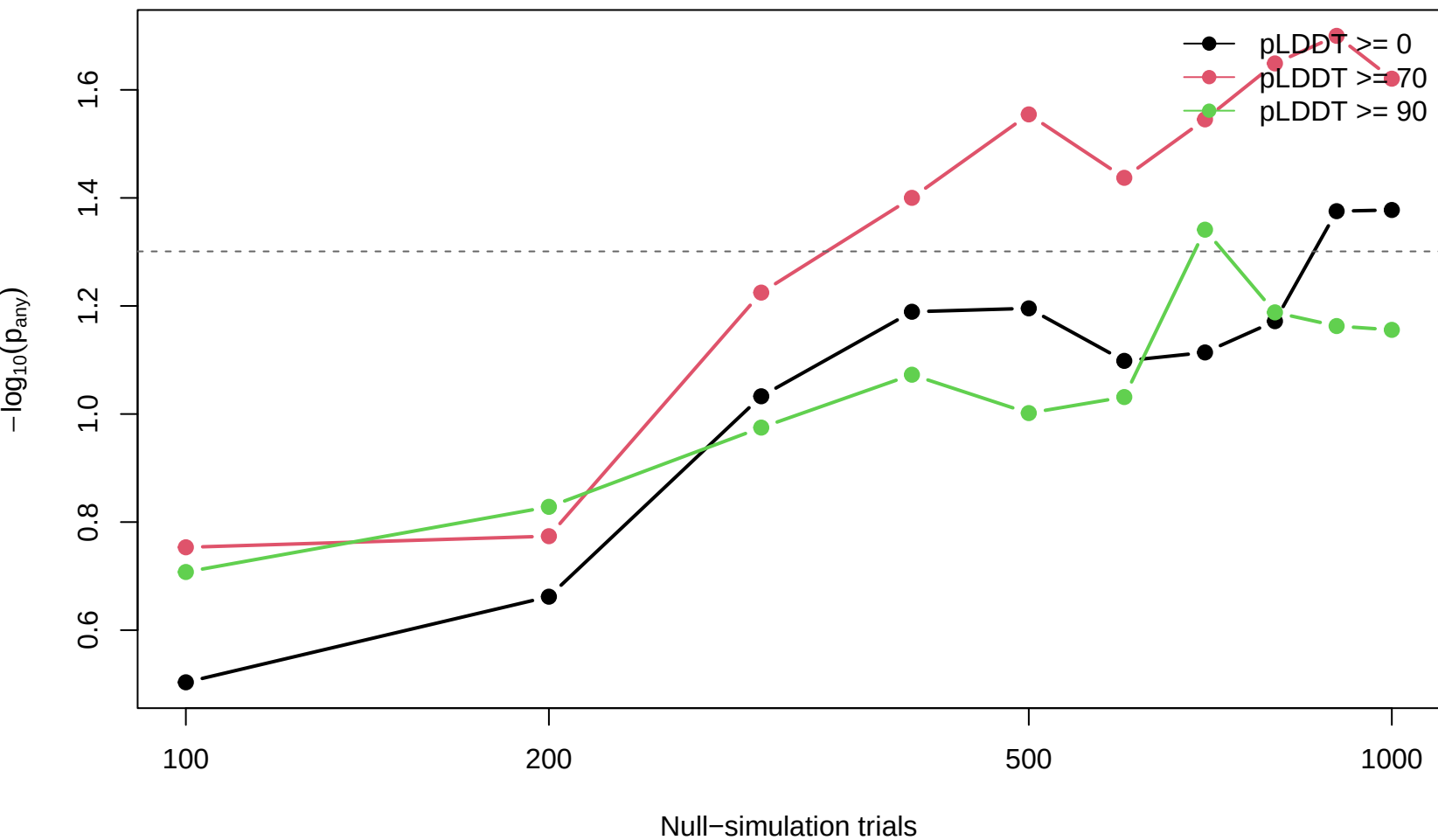
LEF1 cluster_0005 empirical p-value
