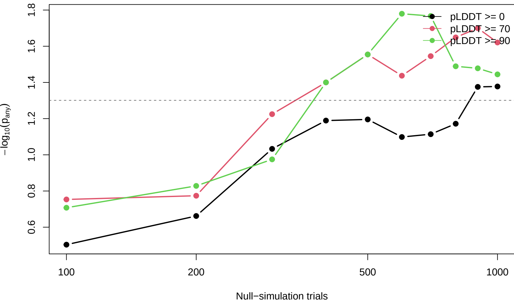
LEF1 cluster_0003 empirical p-value
