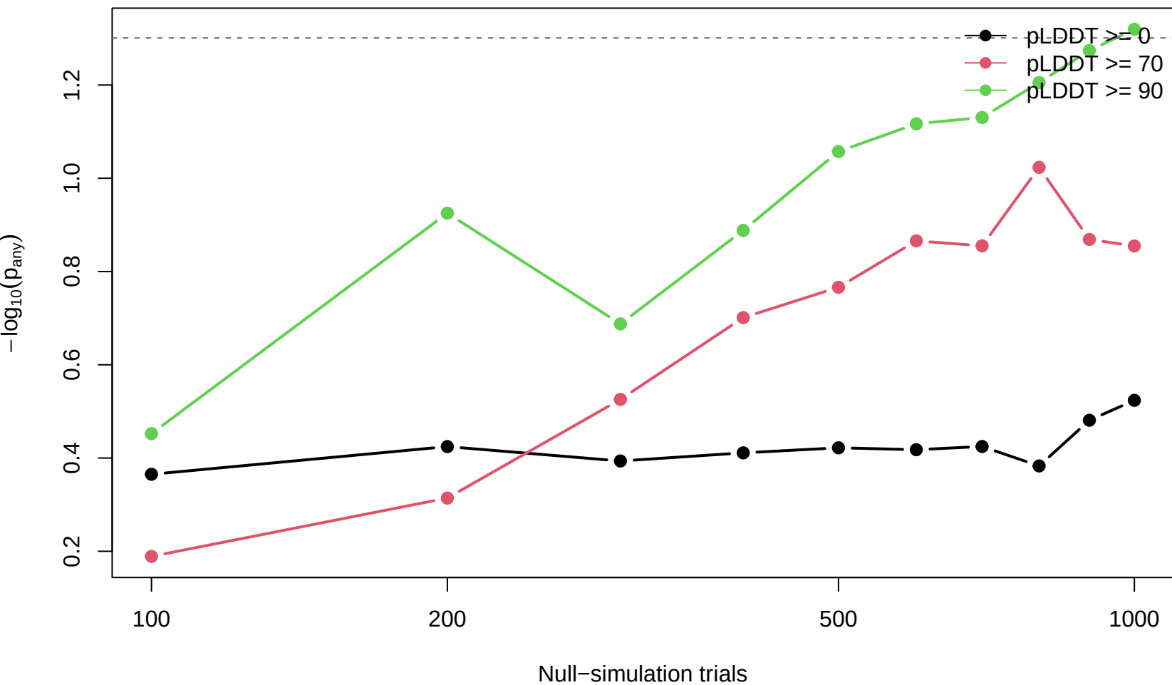
SUZ12 cluster_0004 empirical p-value
