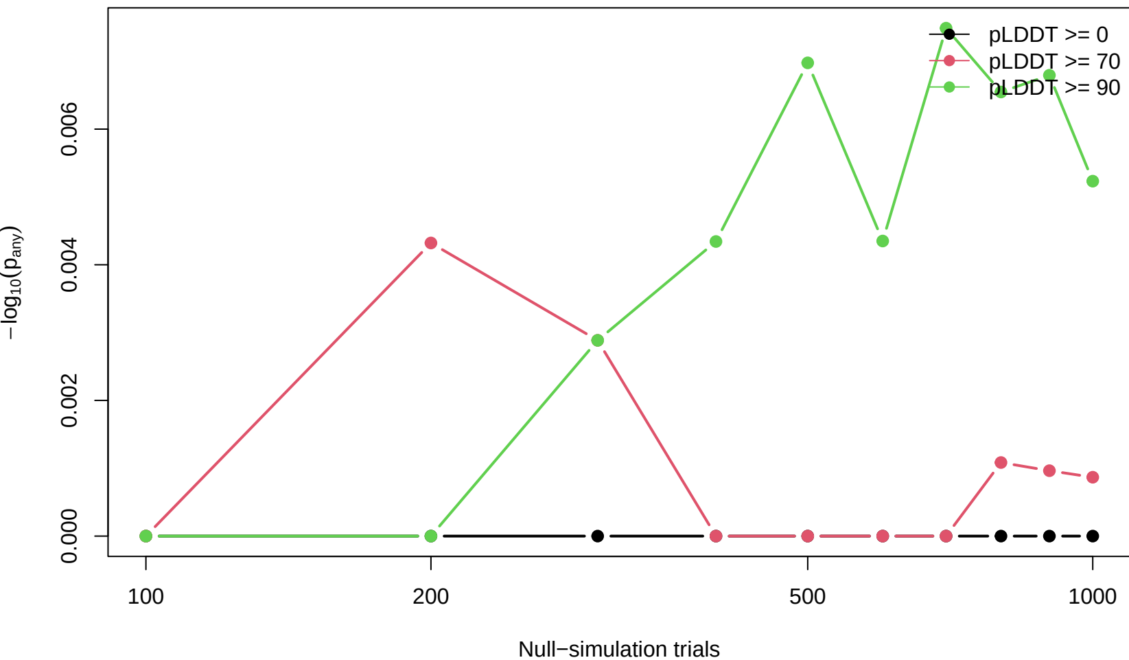
SUZ12 cluster_0064 empirical p-value
