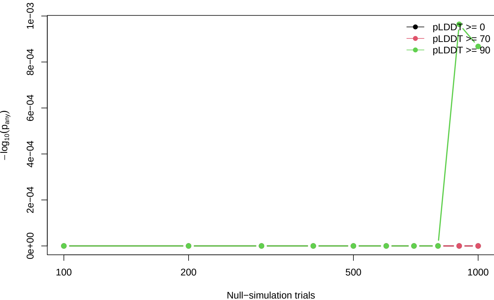
SUZ12 cluster_0072 empirical p-value
