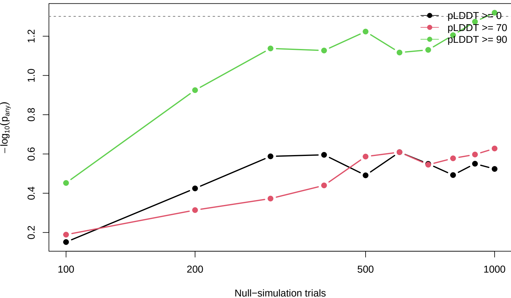
SUZ12 cluster_0003 empirical p-value
