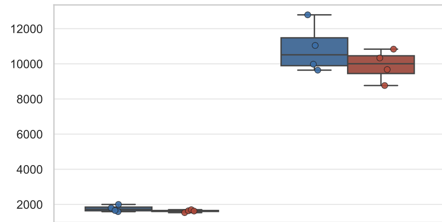
Absolute burden sum log 2 (TPM+1)
