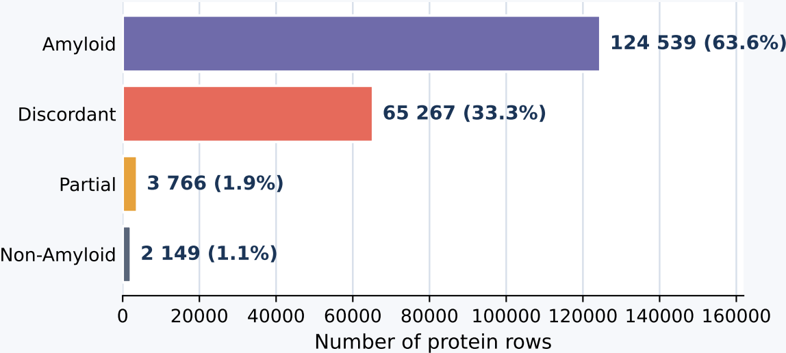
Consensus classes
