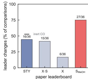
36 comparisons, 19 papers
