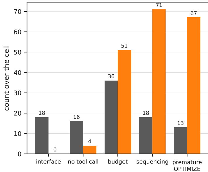
b where the failures moved
