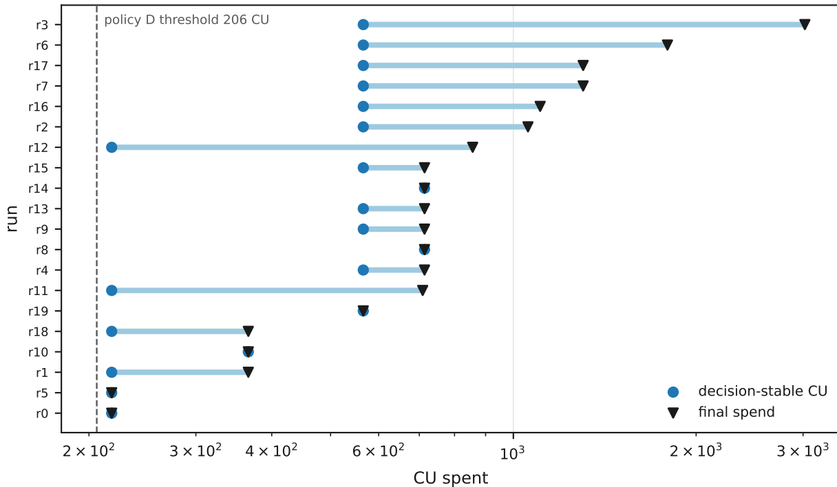
Per-run decision-stable versus final spend, non-binding 5000-CU allowance
