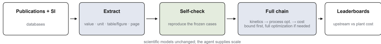
Extraction from 50 papers (recall 97%)
