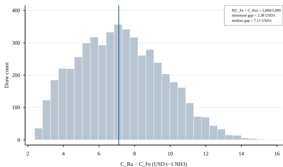
b Joint cost uncertainty does not reverse Fe versus Ru
