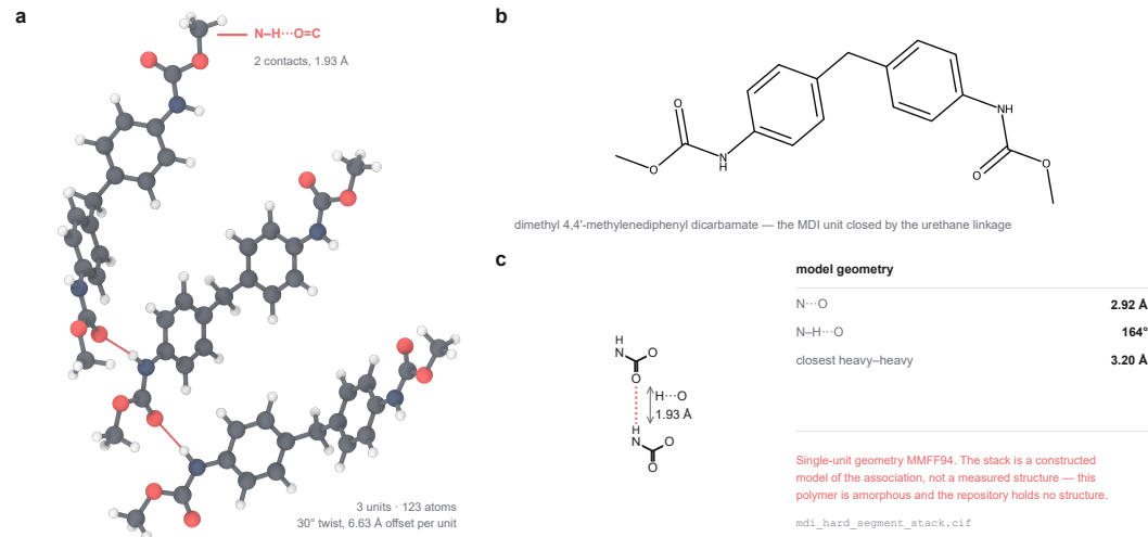
Fig S Hard-segment association, modelled from a generated CIF
