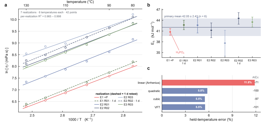
Fig S Viscosity-temperature master panel
