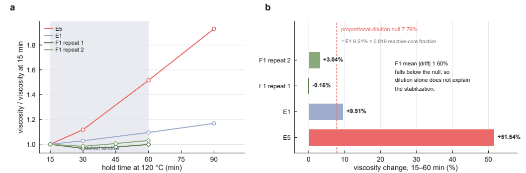
Fig S 120 °C thermal hold against the dilution null
