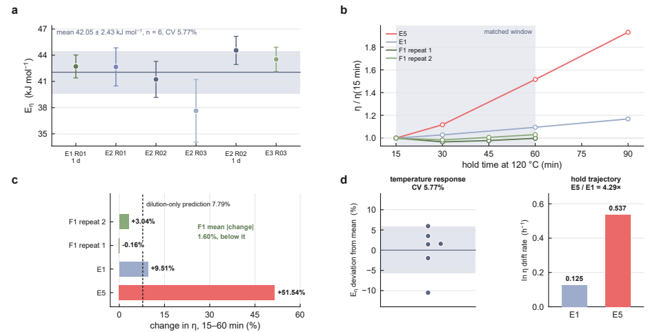
Figure 5 Temperature response is concentrated; hold trajectory is not
