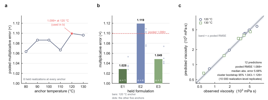
Figure 3 One-point calibration transfers the shared thermal response
