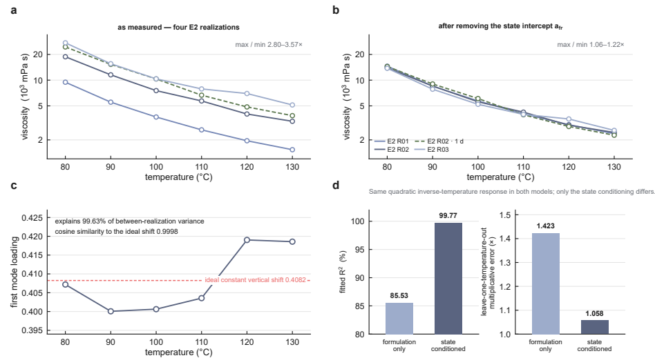
Figure 2 Realization-dependent variation is a calibratable state shift
