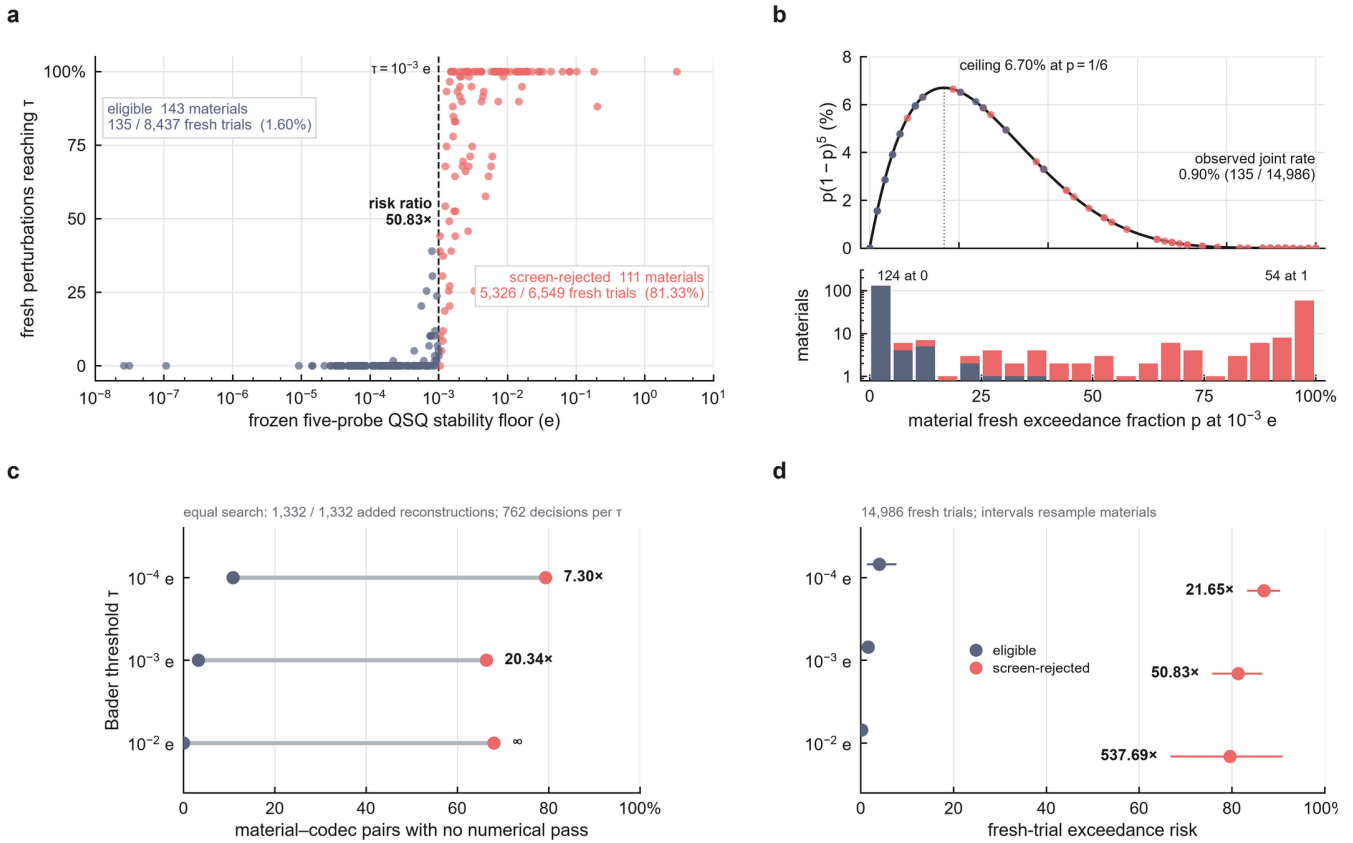
Fig. 2 | The frozen QSQ screen prospectively stratifies downstream numerical risk. a , Each of the 254 development materials at its frozen five-probe stability floor against the fraction of its 59 fresh perturbations whose re-derived Bader response reaches \tau=10^{-3} e (dashed line). The 143 admitted materials (navy) exceed \tau in 135 of 8,437 fresh trials (1.600%; material-cluster 95% CI 0.782–2.596%); the 111 rejected materials (red) in 5,326 of 6,549 (81.325%; 75.981–86.257%). b , Finite-panel admission bound p(1-p)^5 (ceiling 6.70% at p=1/6 ) with every material placed at its fresh exceedance fraction; the observed joint rate is 0.90% (135/14,986). c , Equal-search control: after completing the same tight settings for every material (1,332/1,332 added reconstructions), no-pass risk of eligible and rejected material-codec pairs (762 decisions per threshold); 20.34-fold at 10^{-3} e (3.3% versus 66.4%). d , Fresh exceedance risk at the three pre-specified thresholds with material-cluster 95% intervals: 4.016% versus 86.938% at 10^{-4} e , 1.600% versus 81.325% at 10^{-3} e and 0.148% versus 79.593% at 10^{-2} e .
