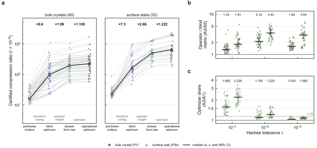
Fig. 6 | The gain ladder separates transform coding, the operator weight and the optimizer. Fresh cohorts as in Fig. 5. a , Certified CR at a Hartree tolerance of 10^{-6} for each material (thin lines) and the median (bold) along the arms: best pointwise codec (A6), operator-blind rate-distortion optimum (A5), closed-form law (A1) and operational optimum in the operator metric (A3); the factor between rungs is the median per-material ratio. b , A3/A5, the operator metric at equal optimization, per material at three tolerances; bar, median; whisker, bootstrap 95% CI (at 10^{-6} : 2.12-fold, 60/60; 3.43-fold, 32/32). c , A3/A1, the optimizer's share over the law; dashed line, pre-registered threshold 1.15 (at 10^{-6} : bulk 1.105, 95% CI 1.090–1.146; slabs 1.222, 1.138–1.359).
