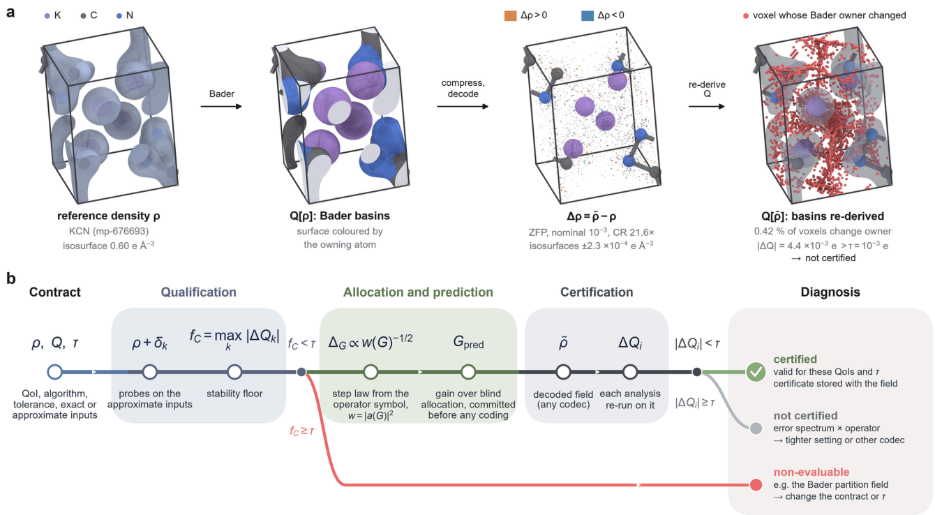
Fig. 1 | The downstream operator at each stage of certified compression. a , The objects the contract acts on for one development material and one frozen benchmark row (KCN, mp-676693; ZFP at nominal relative tolerance 10^{-3} , compression ratio 21.6): reference valence density (isosurface 0.60 \text{ e } \text{\AA}^{-3} ), its Bader basins coloured by owning atom, the decoded error \rho - \tilde{\rho} (isosurfaces \pm 2.3 \times 10^{-4} \text{ e } \text{\AA}^{-3} ) and the voxels whose Bader owner changes when basins are re-derived on \tilde{\rho} (0.42%). The charge error, 4.4 \times 10^{-3} \text{ e} , exceeds \tau = 10^{-3} \text{ e} for a material whose stability floor ( 2.2 \times 10^{-5} \text{ e} ) makes it eligible, so the row is eligible and not certified. b , The workflow as one track. The contract declares the quantity of interest Q , the downstream algorithm, the tolerance \tau and which inputs are exact or approximate. Qualification applies the pre-specified probes \delta_k to the approximate inputs and records the stability floor f_C = \max_k |\Delta Q_k| ; a contract with f_C \geq \tau leaves the main line as non-evaluable. Allocation and prediction read the operator symbol a(G) : the step law \Delta G \propto w(G)^{-1/2} with w = |a(G)|^2 , and the gain over operator-blind allocation, G_{\text{pred}} , committed before any coding. Certification re-runs each analysis on the decoded field from any codec: the field is certified when every |\Delta Q_i| < \tau ; an eligible contract with |\Delta Q_i| \geq \tau at every evaluated setting is not certified.
