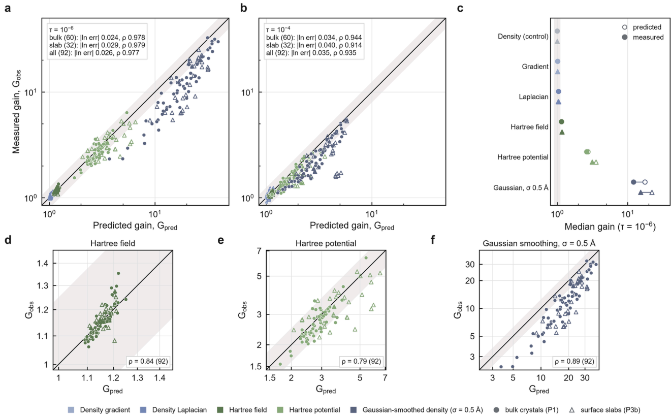
Fig. 8 | The gain of operator-aware allocation is predicted before compression. Five operators (gradient, Laplacian, Hartree field, Hartree potential, Gaussian smoothing with \sigma=0.5 \text{ \AA} ) on 60 fresh bulk crystals (circles) and 32 fresh surface slabs (triangles); predictions were committed before any compression run (P1 d5fc30b, P3b c1e6564). a , Predicted against measured gain at \tau=10^{-6} for 300 bulk and 160 slab material-operator pairs; line, identity; band, \pm 25\% . Median absolute log error 0.024 (bulk), 0.029 (slab), 0.026 (pooled); Spearman 0.978, 0.979 and 0.977. b , The same at \tau=10^{-4} (0.034, 0.040, 0.035; Spearman 0.944, 0.914, 0.935). c , Per-operator medians at \tau=10^{-6} , predicted (open) and measured (filled), bulk (circles) and slab (triangles), ordered by predicted gain, with the density control and the pre-registered null-gain band [0.90, 1.11] (shaded). d–f , Within-operator ranking at \tau=10^{-6} over the 92 materials for the three operators that gain (Spearman 0.84, 0.79 and 0.89).
