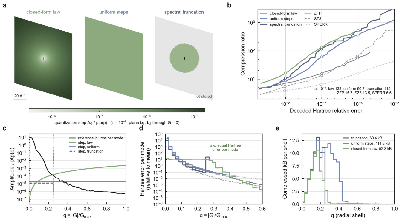
Fig. 4 | The operator symbol fixes where the step, the error and the bytes go. One development density (KCN, mp-676693) and the Hartree potential; every stream is decoded and its Hartree error recomputed. a , Quantization step \Delta G on the reciprocal plane through G=0 spanned by b_1 and b_2 for the closed-form law ( \Delta G \propto |G|^2 ), uniform steps and spectral truncation at its best cutoff ( q=0.25 ; outer modes not stored), each at its certified point for a Hartree tolerance of 10^{-6} ; G=0 (cross) is stored exactly. b , Compression ratio against decoded Hartree relative error; truncation is the lower envelope over 32 cutoffs; open circles, certified points at 10^{-4} , 10^{-6} and 10^{-8} (vertical lines). c , Root-mean-square reference coefficient per radial bin, q=|G|/G_{\max} , and the step of each policy at 10^{-6} . d , Hartree error per mode relative to its all-mode mean, per radial bin, at 10^{-6} ; colours and line styles as in b . e , Compressed bytes per radial shell at 10^{-6} , with stream totals.
