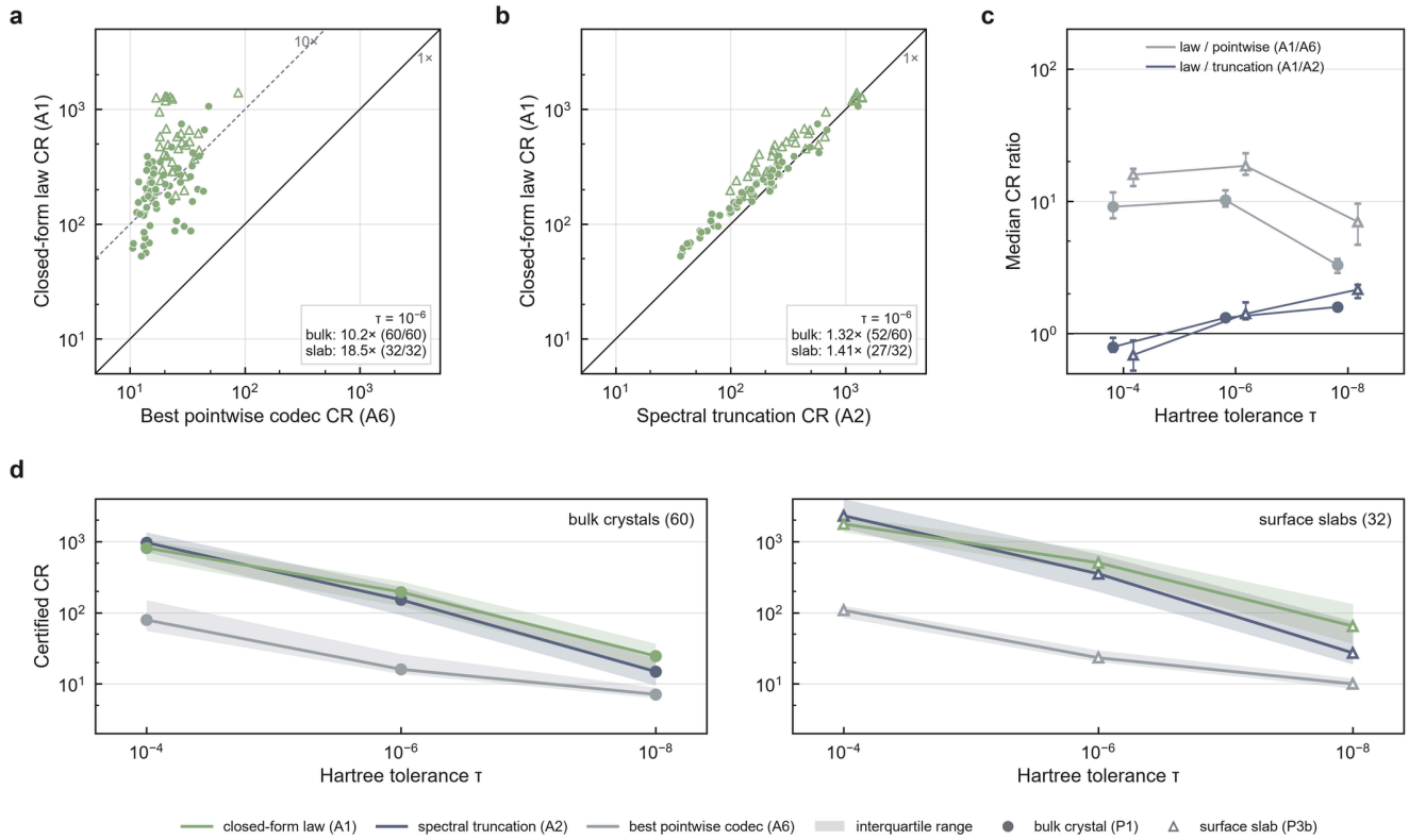
Fig. 5 | Under equal search, the closed-form law certifies an order of magnitude more than pointwise codecs and beats spectral truncation. Fresh cohorts: 60 bulk crystals (P1, circles) and 32 surface slabs (P3b, triangles); every stream decode-verified; A1, A2 and A6 receive equal continuous search. a , Certified compression ratio (CR) of the law (A1) against the best of ZFP, SZ3 and SPERR (A6) at Hartree relative error 10^{-6} ; lines mark ratios 1 and 10 (medians 10.2-fold, 60/60, and 18.5-fold, 32/32). b , A1 against spectral truncation (A2) at 10^{-6} (1.32-fold, 52/60; 1.41-fold, 27/32). c , Median ratios A1/A6 and A1/A2 with bootstrap 95% CIs at 10^{-4} , 10^{-6} and 10^{-8} for each cohort. d , Certified CR against tolerance for the three arms: median (line) and interquartile range (band) over the materials of each cohort.
