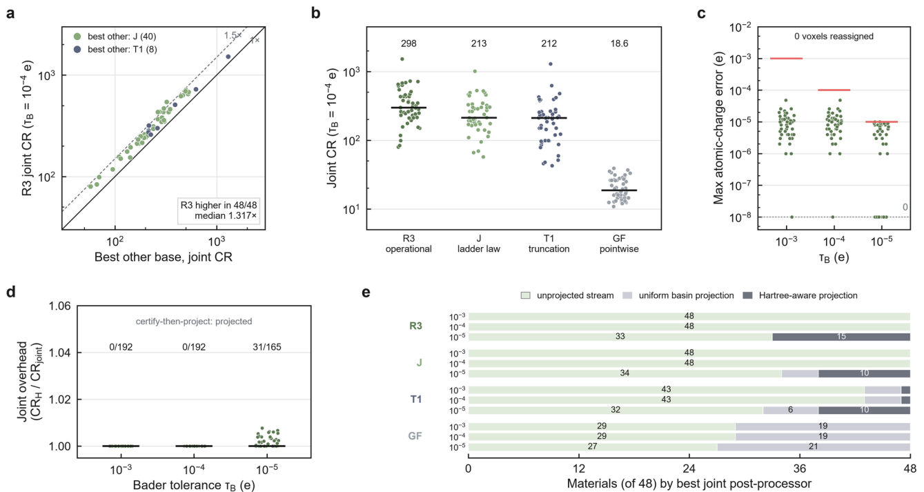
Fig. 7 | One operator-aware stream certifies the Hartree potential and Bader charges together. 48 fresh bulk crystals (P2); joint contract: Hartree relative error below 10^{-6} and Henkelman Bader charges with an exact all-electron partition reference, error at most \tau_B , zero basin reassignment. a , Joint compression ratio of the operational Hartree encoder (R3) against the best other base codec for each material at \tau_B = 10^{-4} e, coloured by that base; R3 is higher in 48/48 (median 1.317-fold). b , Joint CR at \tau_B = 10^{-4} e for each base codec at its best post-processor: R3, frozen-ladder law (J), spectral truncation (T1) and pointwise codecs (GF) (medians 298, 213, 212 and 18.6). c , Maximum atomic-charge error of the certified R3 stream per material at each \tau_B (red bars, \tau_B ); errors of exactly zero are drawn on the dashed floor; no voxel was reassigned (144/144). d , Joint overhead (Hartree-only over joint CR) of R3 at each \tau_B (median 1.000 at each), with the number of certify-then-project decisions that applied a projection (0/192, 0/192, 31/165). e , Post-processor that gave each base its best joint stream at each \tau_B .
