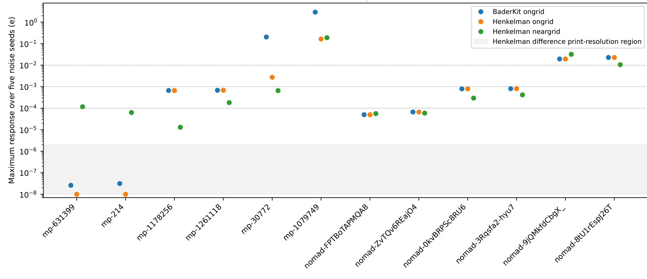
Independent-method perturbation response | 12 selected development systems
