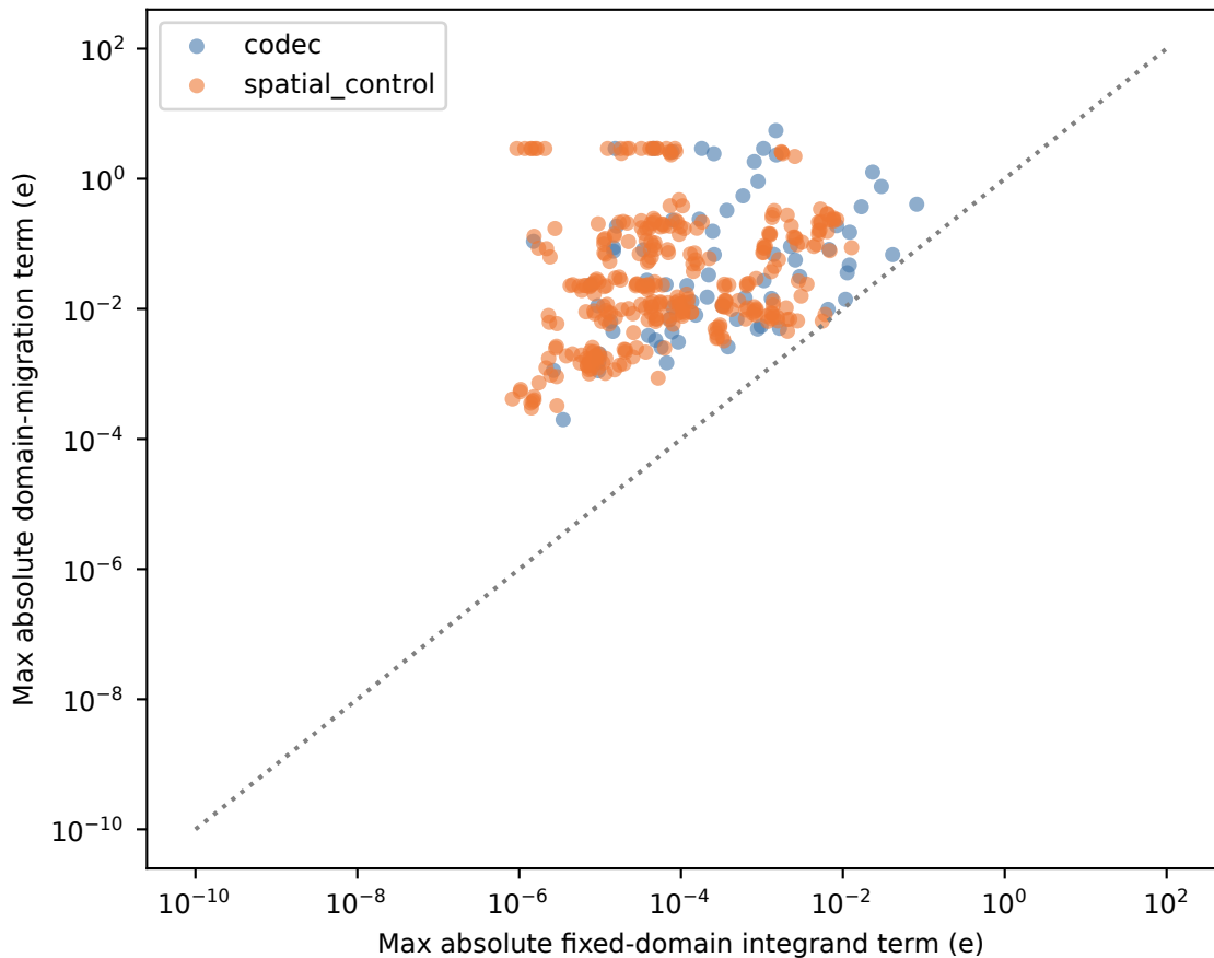
BaderKit exact per-atom charge decomposition
