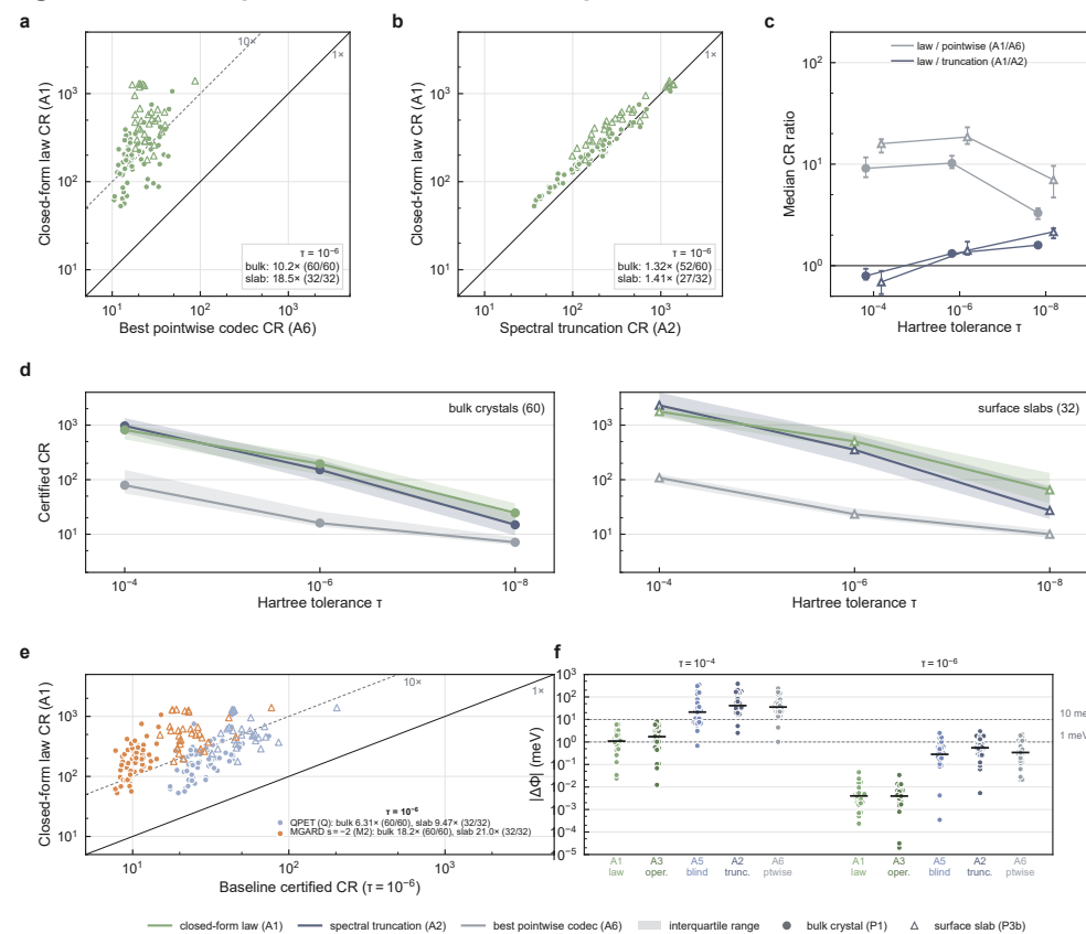
Figure 5 Under equal search the law beats pointwise codecs and truncation
