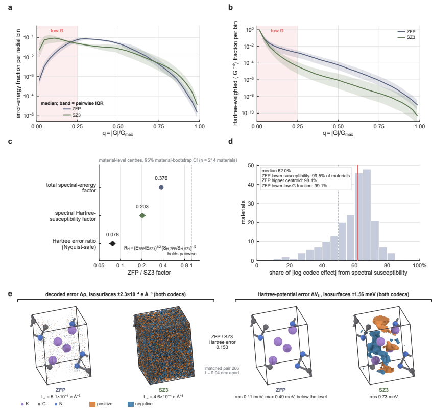
Figure 3 The Hartree operator's spectral weight explains the codec effect
