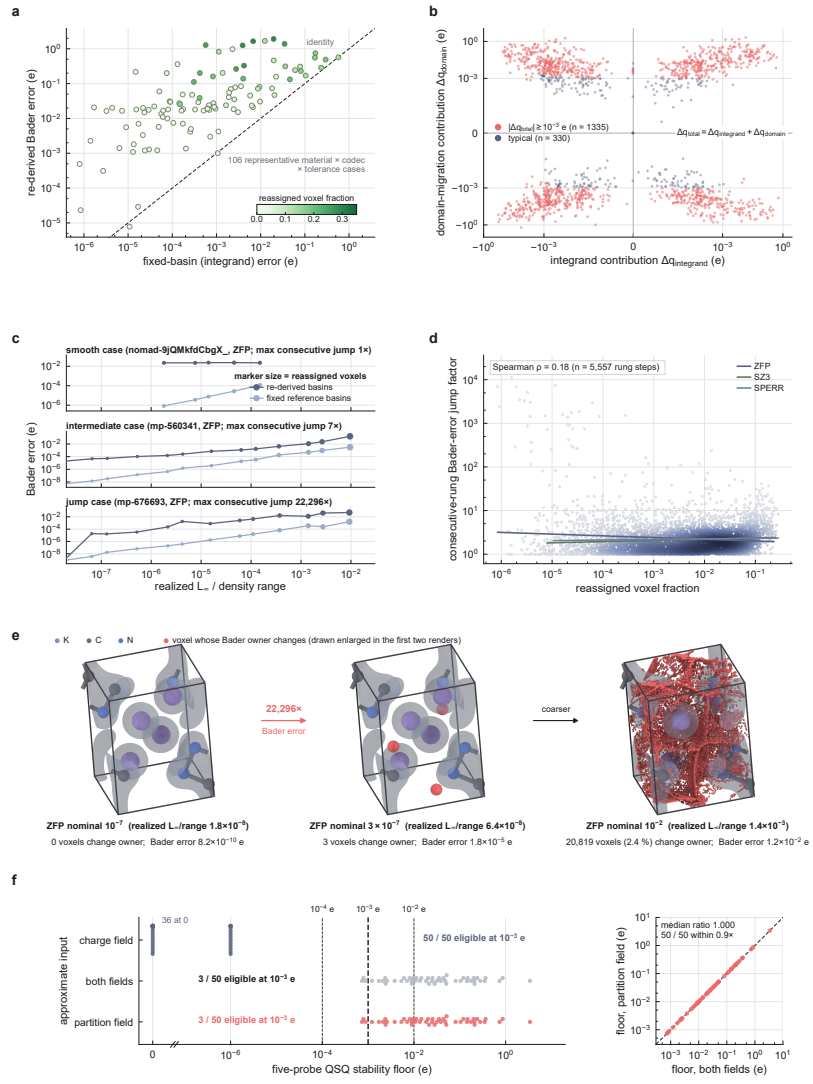
Figure 5 Partition-field basin migration explains Bader instability
