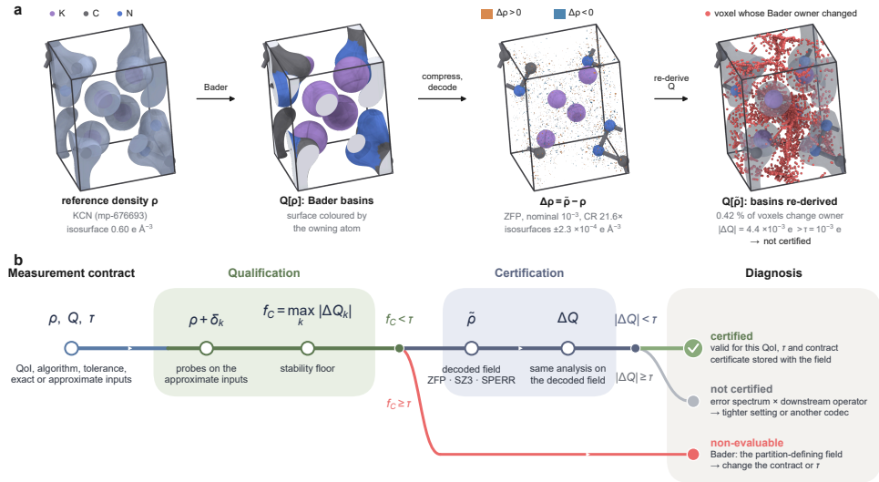
Figure 1 Qualification, certification and diagnosis of a measurement contract
