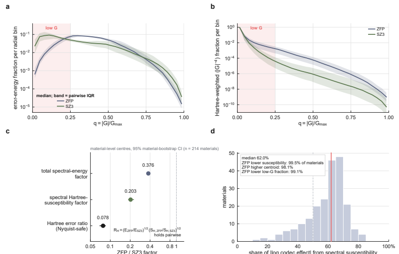
Figure 7 Frequency allocation of error controls Hartree fidelity
