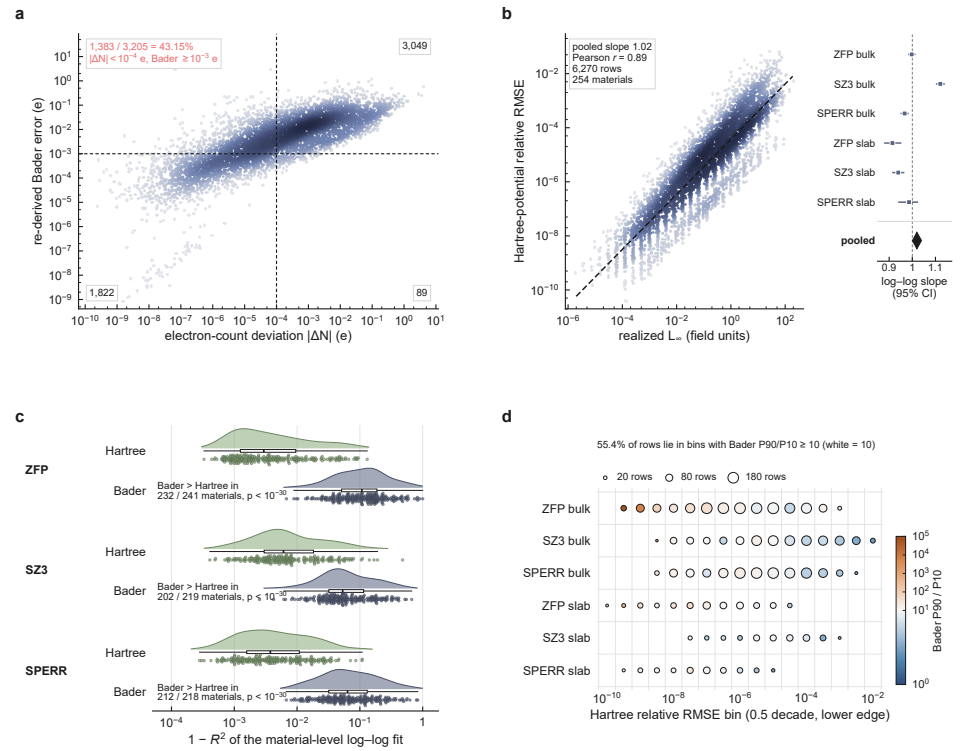
Figure 2 Downstream operator structure controls error propagation
