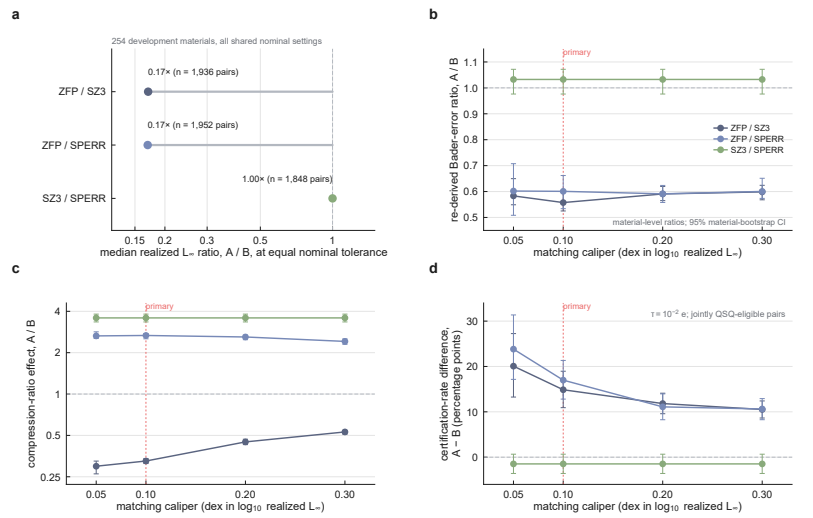
Figure 6 Equal nominal tolerance conflates distortion with error structure
