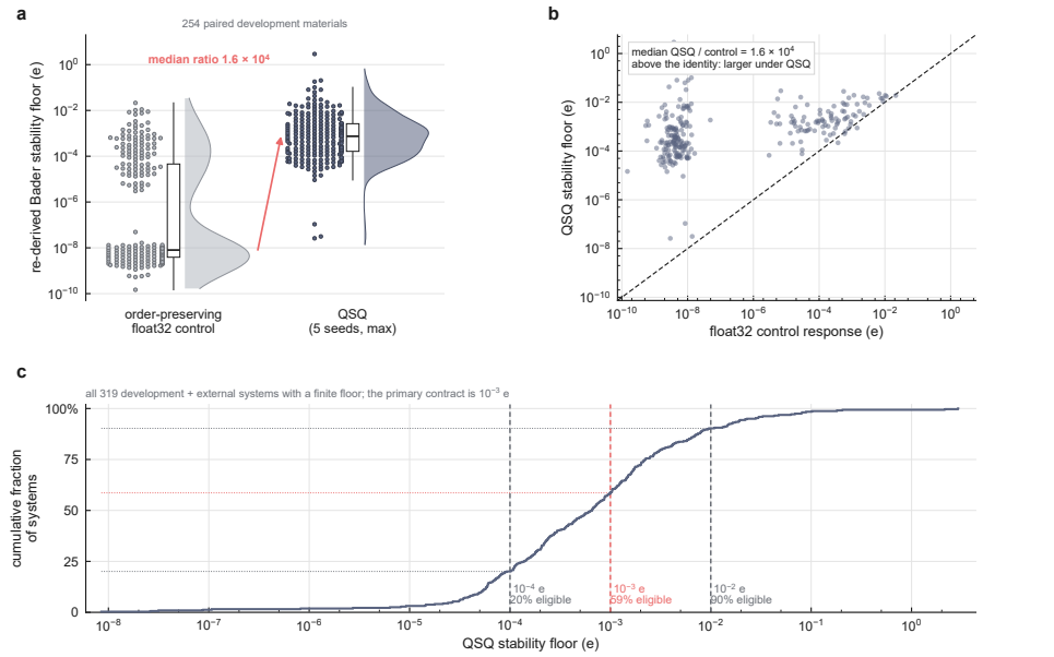
Figure 4 A stability probe must excite the numerical failure mode
