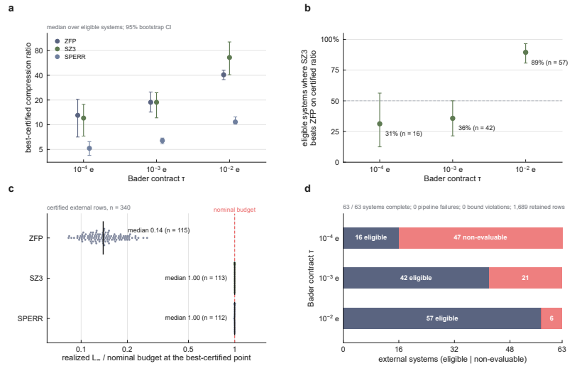
Figure 8 Untouched external systems reproduce the decision frontier
