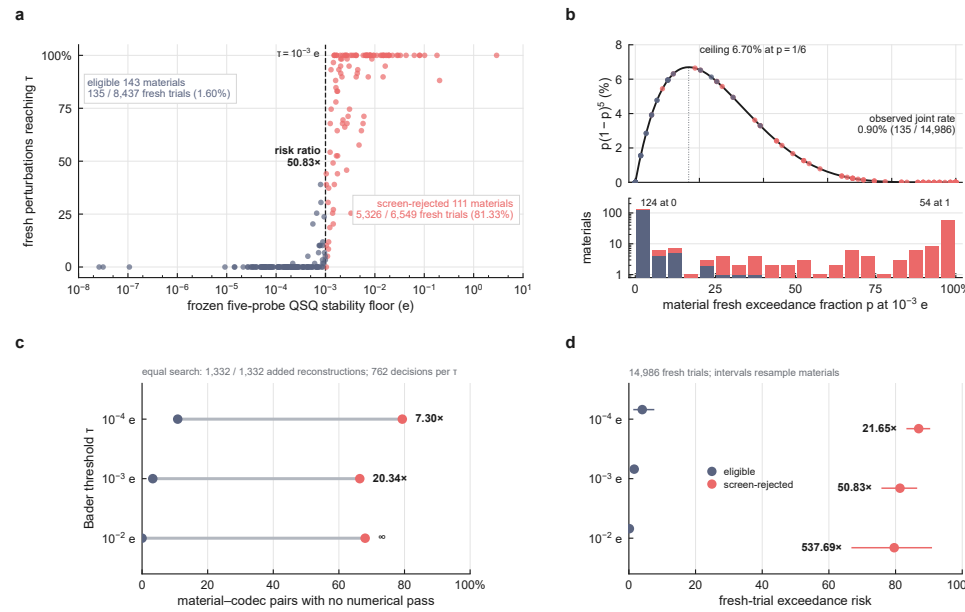
Figure 3 The frozen QSQ screen prospectively stratifies numerical risk
