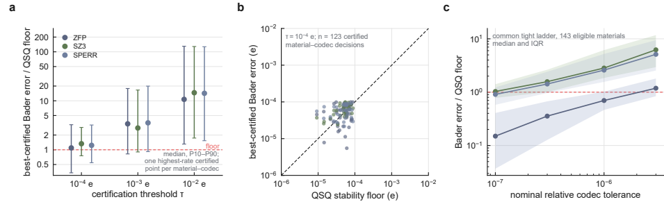
Figure S4 The strictest certified regime is floor-scale
