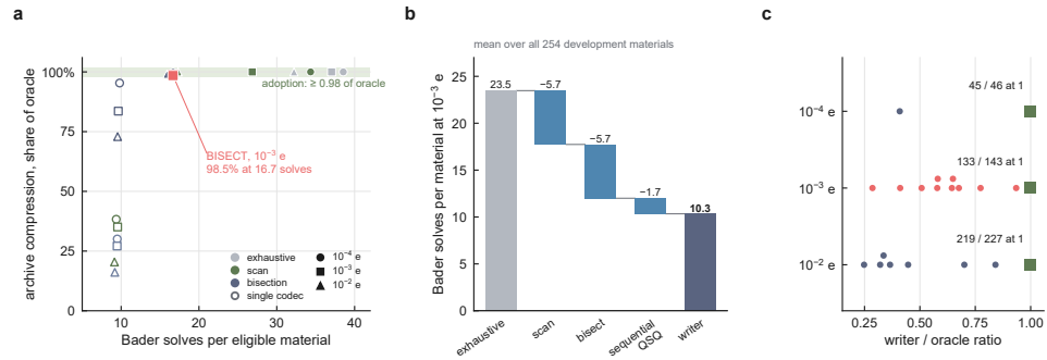
Figure S10 A certifying writer at a fraction of the exhaustive cost
