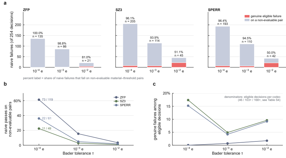
Figure S7 Codec-resolved consequences of qualification
