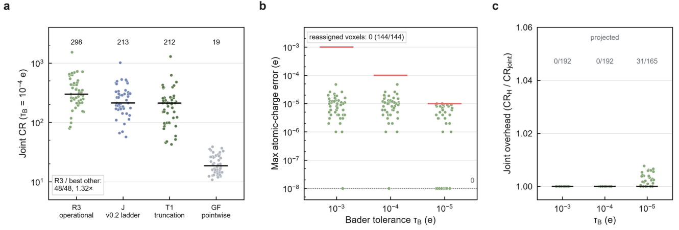
Fig. 6 | One operator-aware stream certifies the Hartree potential and Bader charges together. 48 fresh bulk crystals (P2); joint contract: Hartree relative error below 10^{-6} and Henkelman Bader charges with an exact all-electron partition reference, error at most \tau_B , zero basin reassignment. a , Joint compression ratio at \tau_B=10^{-4} e for each base codec at its best post-processor: operational Hartree encoder (R3), frozen-ladder law (J), spectral truncation (T1) and pointwise codecs (GF) (medians 298, 213, 212 and 18.6; R3 best in 48/48, median 1.317-fold over the best other base). b , Maximum atomic-charge error of the certified R3 stream per material at each \tau_B (red bars, \tau_B ); errors of exactly zero are drawn on the dashed floor; no voxel was reassigned (144/144). c , Joint overhead (Hartree-only over joint compression ratio) of R3 at each \tau_B (median 1.000 at each), with the number of certify-then-project decisions that applied a projection (0/192, 0/192, 31/165).
