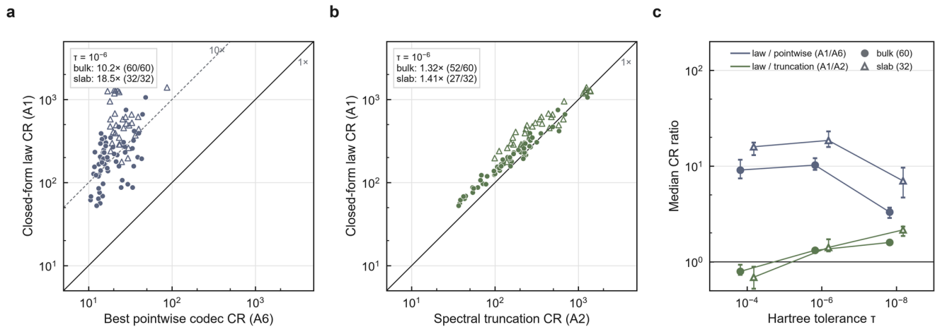
Fig. 4 | Under equal search, the closed-form law certifies an order of magnitude more than pointwise codecs and beats spectral truncation. Fresh cohorts: 60 bulk crystals (P1, circles) and 32 surface slabs (P3b, triangles); every stream decode-verified; A1, A2 and A6 receive equal continuous search. a , Certified compression ratio (CR) of the law (A1) against the best of ZFP, SZ3 and SPERR (A6) at Hartree relative error 10^{-6} ; lines mark ratios 1 and 10 (medians 10.2-fold, 60/60, and 18.5-fold, 32/32). b , A1 against spectral truncation (A2) at 10^{-6} (1.32-fold, 52/60; 1.41-fold, 27/32). c , Median ratios A1/A6 and A1/A2 with bootstrap 95% CIs at 10^{-4} , 10^{-6} and 10^{-8} for each cohort.
