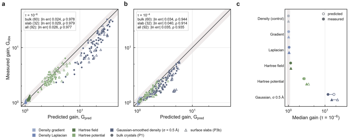
Fig. 7 | The gain of operator-aware allocation is predicted before compression. Five operators (gradient, Laplacian, Hartree field, Hartree potential, Gaussian smoothing with \sigma=0.5 \text{ \AA} ) on 60 fresh bulk crystals (circles) and 32 fresh surface slabs (triangles); predictions were committed before any compression run (P1 d5fc30b, P3b c1e6564). a , Predicted against measured gain at \tau=10^{-6} for 300 bulk and 160 slab material-operator pairs; line, identity; band, \pm 25\% . Median absolute log error 0.024 (bulk), 0.029 (slab), 0.026 (pooled); Spearman 0.978, 0.979 and 0.977. b , The same at \tau=10^{-4} (0.034, 0.040, 0.035; Spearman 0.944, 0.914, 0.935). c , Per-operator medians at \tau=10^{-6} , predicted (open) and measured (filled), bulk (circles) and slab (triangles), ordered by predicted gain, with the density control and the pre-registered null-gain band [0.90, 1.11] (shaded).
