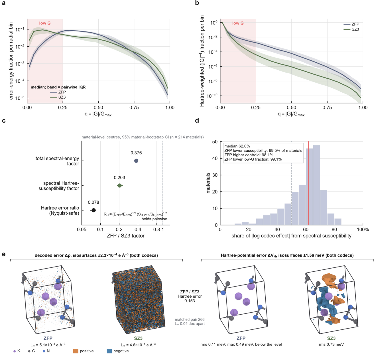
Fig. 3 | The Hartree operator's spectral weight explains the codec effect at matched distortion. a , Radial reconstruction-error spectra for the 457 within-material ZFP/SZ3 pairs matched on realized L_\infty (214 materials); medians of non-zero, Nyquist-safe error-energy fractions with pairwise interquartile ribbons. b , Hartree weighting ( |G|^{-4} ) emphasizes the long-wavelength modes where SZ3 places more error. c , Material-level centres and 95% bootstrap intervals of the total spectral-energy factor (0.376), the Hartree-susceptibility factor (0.203) and the Nyquist-safe Hartree-error ratio (0.07762); the multiplicative closure is exact for each pair. d , The susceptibility factor contributes a material-median 62.0% of the absolute log codec effect. e , One matched pair in three dimensions (KCN, mp-676693): at one decoded-error isolevel, ZFP error is confined to sparse voxels whereas SZ3 error fills the cell, and the Hartree-potential error forms long-wavelength SZ3 lobes that ZFP does not reach (RMS 0.11 versus 0.73 meV).
