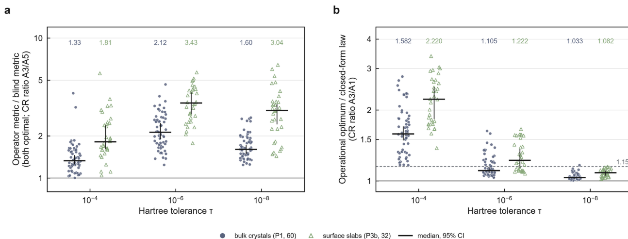
Fig. 5 | The operator metric carries the gain; the optimizer's share is set by the system class. Per material (points), median (bar) and bootstrap 95% CI (whisker) at three Hartree tolerances; bulk crystals (60) and surface slabs (32). a , Operational optimum under the operator metric (A3) over the same optimum under the blind L_2 metric (A5), both certified for the same Hartree contract (at 10^{-6} : 2.12-fold, 60/60; 3.43-fold, 32/32). b , Operational optimum over the closed-form law (A3/A1); dashed line, pre-registered threshold 1.15. At 10^{-6} the law is within 10.5% of the optimum for bulk crystals (median 1.105, 95% CI 1.090–1.146) and operational allocation adds 22% for slabs (1.222, 1.138–1.359).
