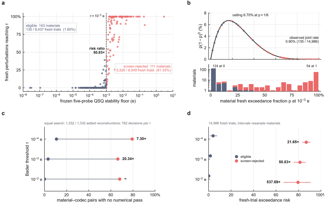
Fig. 2 | The frozen QSQ screen prospectively stratifies downstream numerical risk. a , Each of the 254 development materials at its frozen five-probe stability floor against the fraction of its 59 fresh perturbations whose re-derived Bader response reaches \tau=10^{-3} e (dashed line). The 143 admitted materials (navy) exceed \tau in 135 of 8,437 fresh trials (1.600%; material-cluster 95% CI 0.782–2.596%); the 111 rejected materials (red) in 5,326 of 6,549 (81.325%; 75.981–86.257%). b , Finite-panel admission bound p(1-p)^5 (ceiling 6.70% at p=1/6 ) with every material placed at its fresh exceedance fraction; the observed joint rate is 0.90% (135/14,986). c , Equal-search control: after completing the same tight settings for every material (1,332/1,332 added reconstructions), no-pass risk of eligible and rejected material-codec pairs (762 decisions per threshold); 20.34-fold at 10^{-3} e (3.3% versus 66.4%). d , Fresh exceedance risk at the three pre-specified thresholds with material-cluster 95% intervals: 4.016% versus 86.938% at 10^{-4} e , 1.600% versus 81.325% at 10^{-3} e and 0.148% versus 79.593% at 10^{-2} e .
