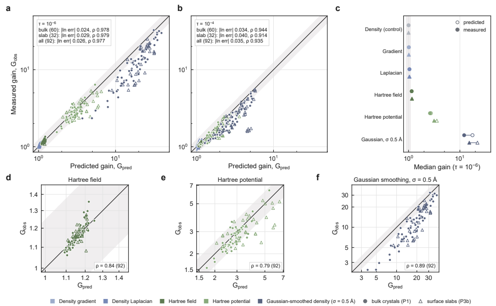
Figure 8 The gain is predicted before compression
