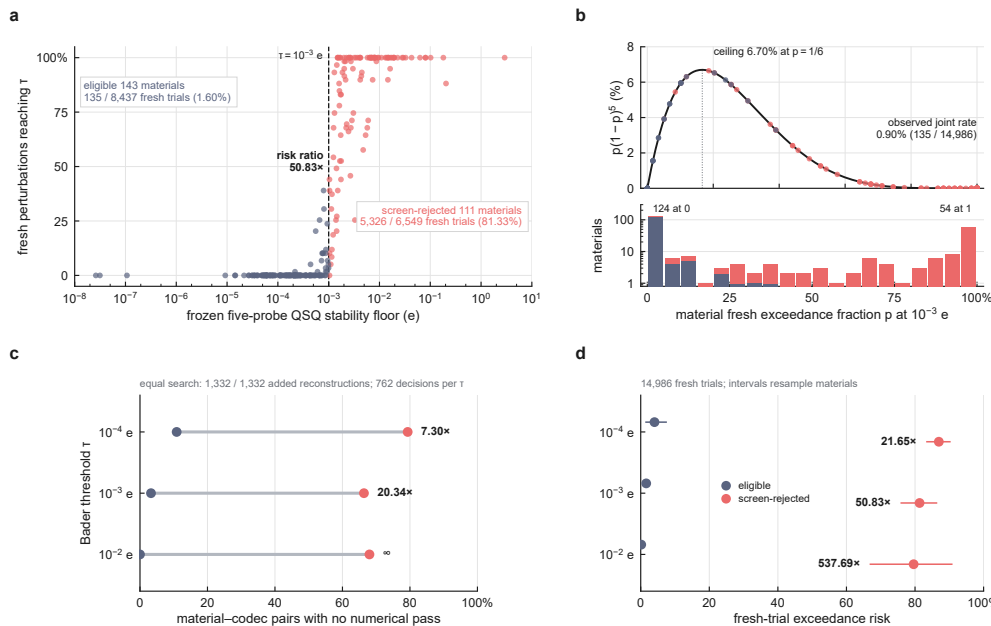
Figure 2 The frozen QSQ screen prospectively stratifies numerical risk
