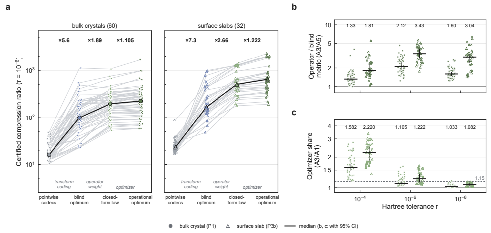
Figure 6 The gain ladder: transform coding, operator weight, optimizer
