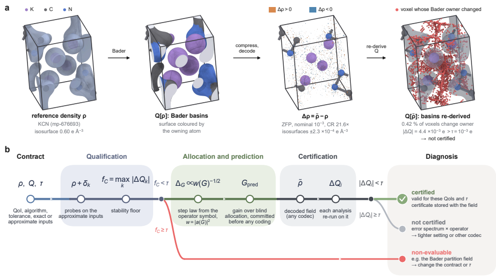
Figure 1 The downstream operator at each stage of certified compression
