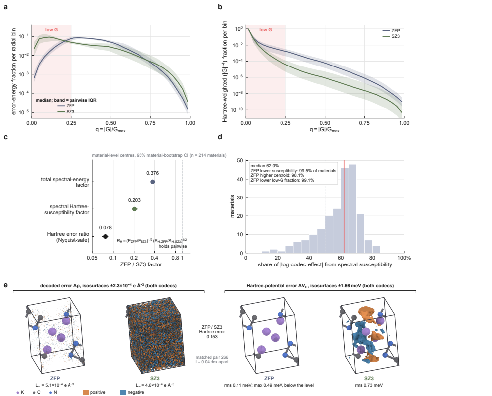
Figure 3 The Hartree operator's spectral weight explains the codec effect
