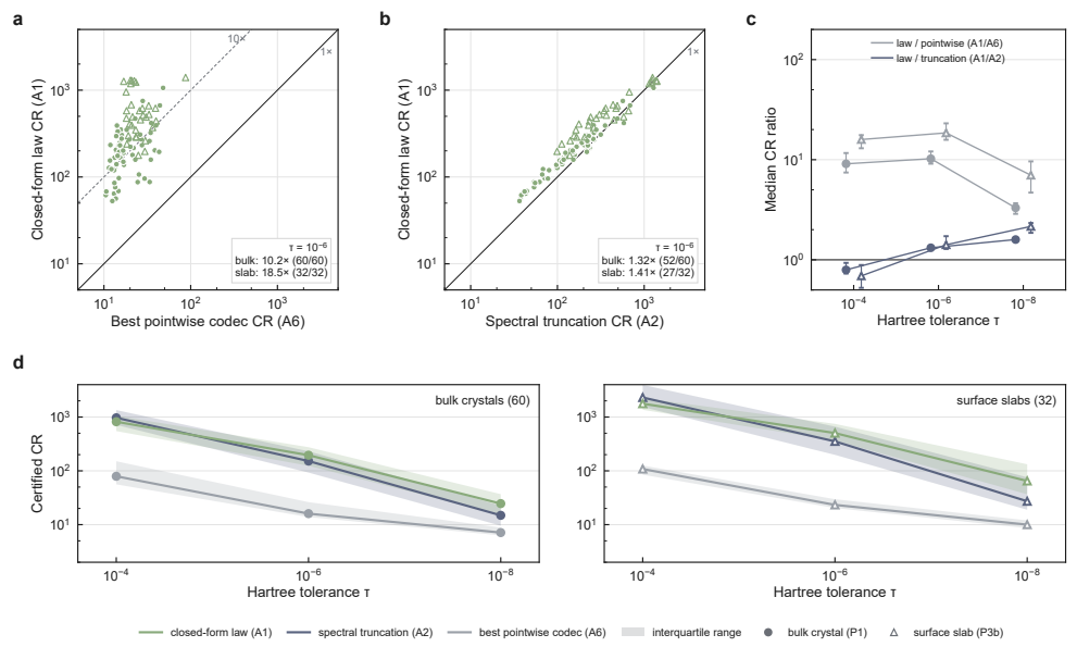
Figure 5 Under equal search the law beats pointwise codecs and truncation
