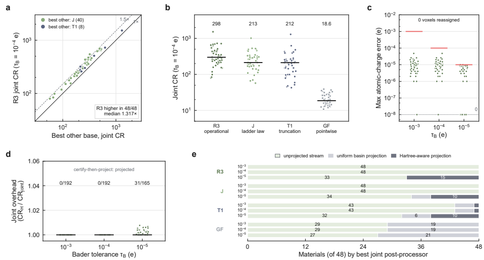
Figure 7 One stream certifies the Hartree potential and Bader charges
