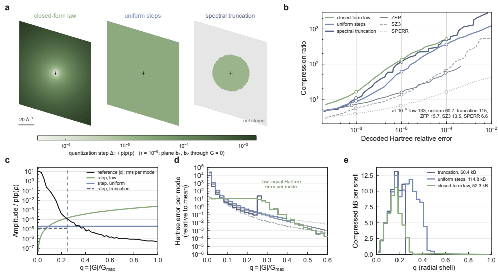
Figure 4 The operator symbol fixes where the step, the error and the bytes go
