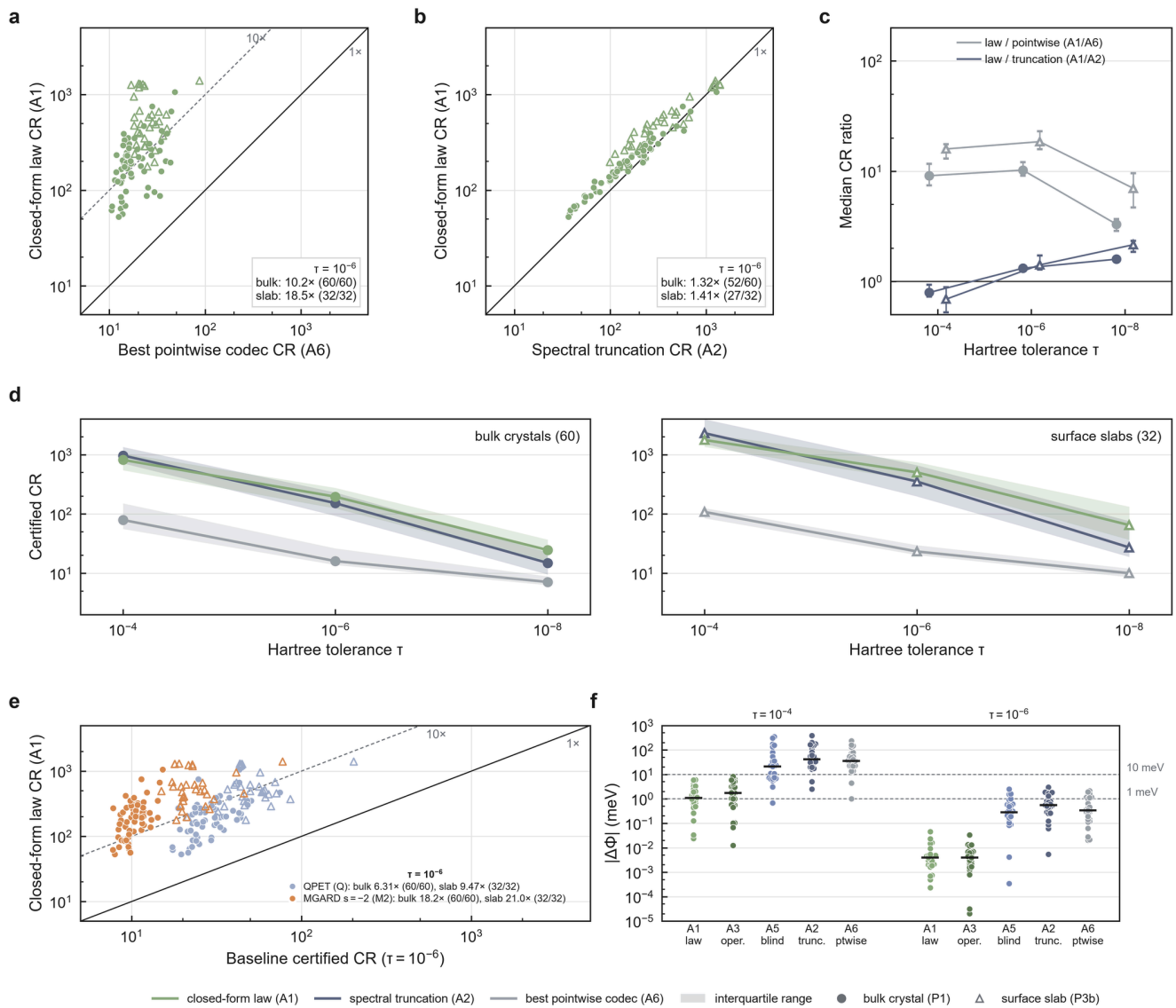
Fig. 5 | Under equal search, the closed-form law certifies more than pointwise and QoI-preserving codecs and preserves slab work functions. Fresh cohorts: 60 bulk crystals (P1, circles) and 32 surface slabs (P3b, triangles); every stream decode-verified; every arm receives equal continuous search. a , Certified compression ratio (CR) of the law (A1) against the best of ZFP, SZ3 and SPERR (A6) at Hartree relative error 10^{-6} ; lines mark ratios 1 and 10 (medians 10.2-fold, 60/60, and 18.5-fold, 32/32). b , A1 against spectral truncation (A2) at 10^{-6} (1.32-fold, 52/60; 1.41-fold, 27/32). c , Median ratios A1/A6 and A1/A2 with bootstrap 95% CIs at 10^{-4} , 10^{-6} and 10^{-8} for each cohort. d , Certified CR against tolerance for the three arms: median (line) and interquartile range (band) over the materials of each cohort. e , A1 against two QoI-preserving compressors at 10^{-6} , QPET bounding a block average of the density (best of nine configurations; blue; medians 6.31-fold, 60/60, and 9.47-fold, 32/32) and MGARD with smoothness s=-2 (orange; 18.2-fold, 60/60, and 21.0-fold, 32/32); lines mark ratios 1 and 10. f , Work-function error |\Delta\Phi| of the certified streams for the 27 slabs with a vacuum region, per arm, at Hartree tolerances 10^{-4} and 10^{-6} . Bars mark medians: A1 1.09 and 0.0040 meV; A6 35.5 and 0.34 meV. Dashed lines mark 1 and 10 meV. A3, operational optimum; A5, operator-blind rate-distortion optimum.
