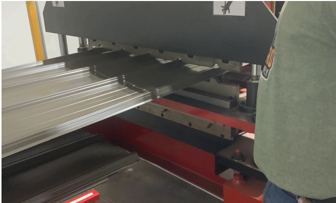
Roll former shear head with yellow safety perimeter rail and CAUTION labels
