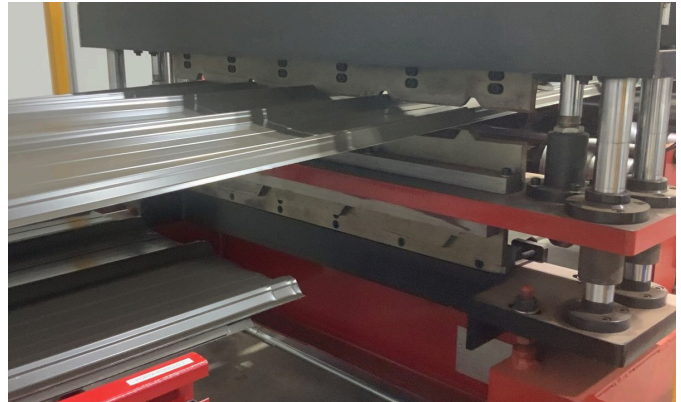
Roll former — yellow safety rail, CAUTION shear labels, panel output visible
