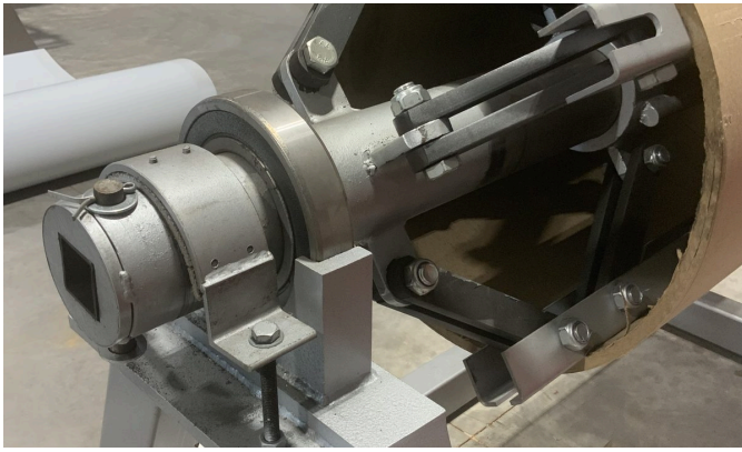
D-coiler mandrel — coil expansion mechanism; machine-specific LOTO procedures documented
