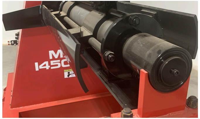
Maber 1450 roll former — forming rollers; CAUTION label affixed by manufacturer
