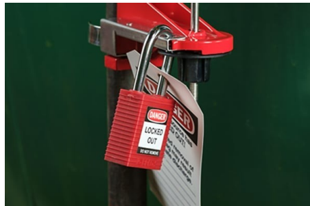
Padlock + "Do Not Operate" tag on the disconnect.
