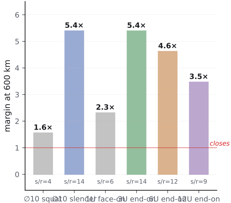
margin by shape (600 km, 100 V drive)
