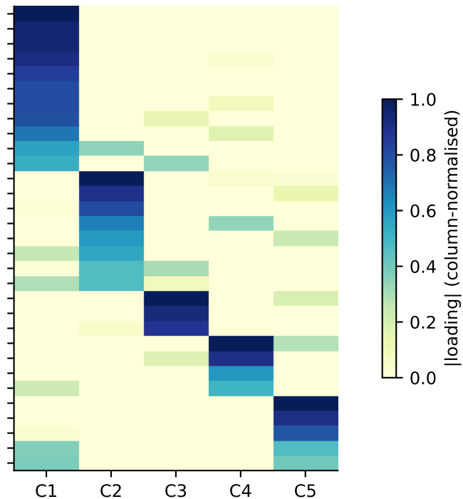
NSA-PCA loadings ( w = 0.9 )
