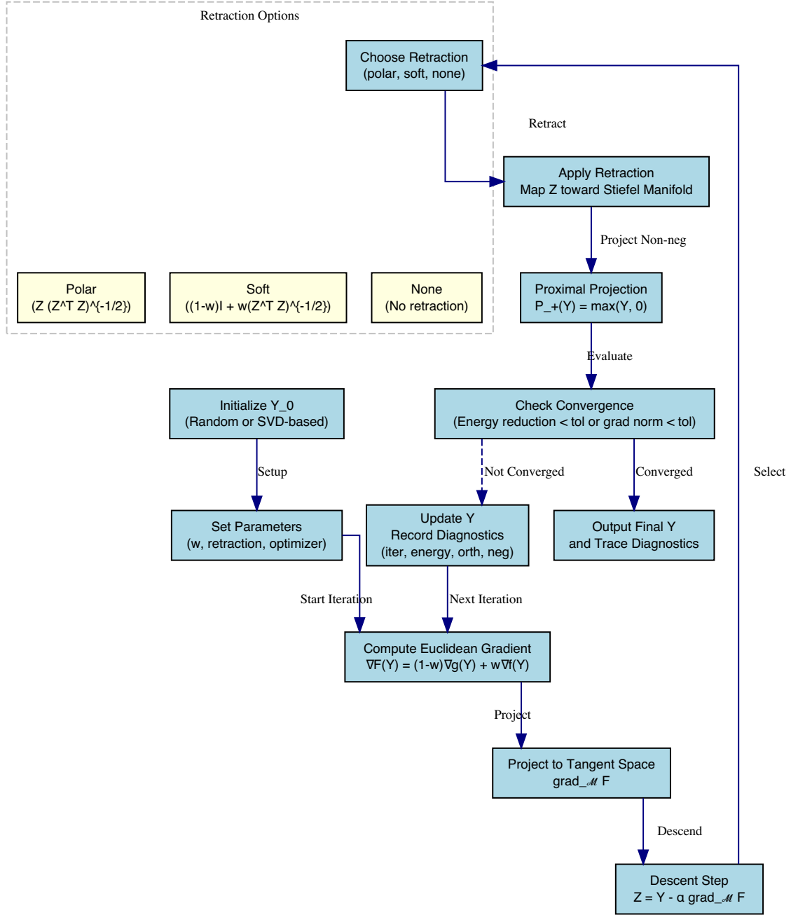
Figure 2: NSA-Flow Algorithm Workflow
