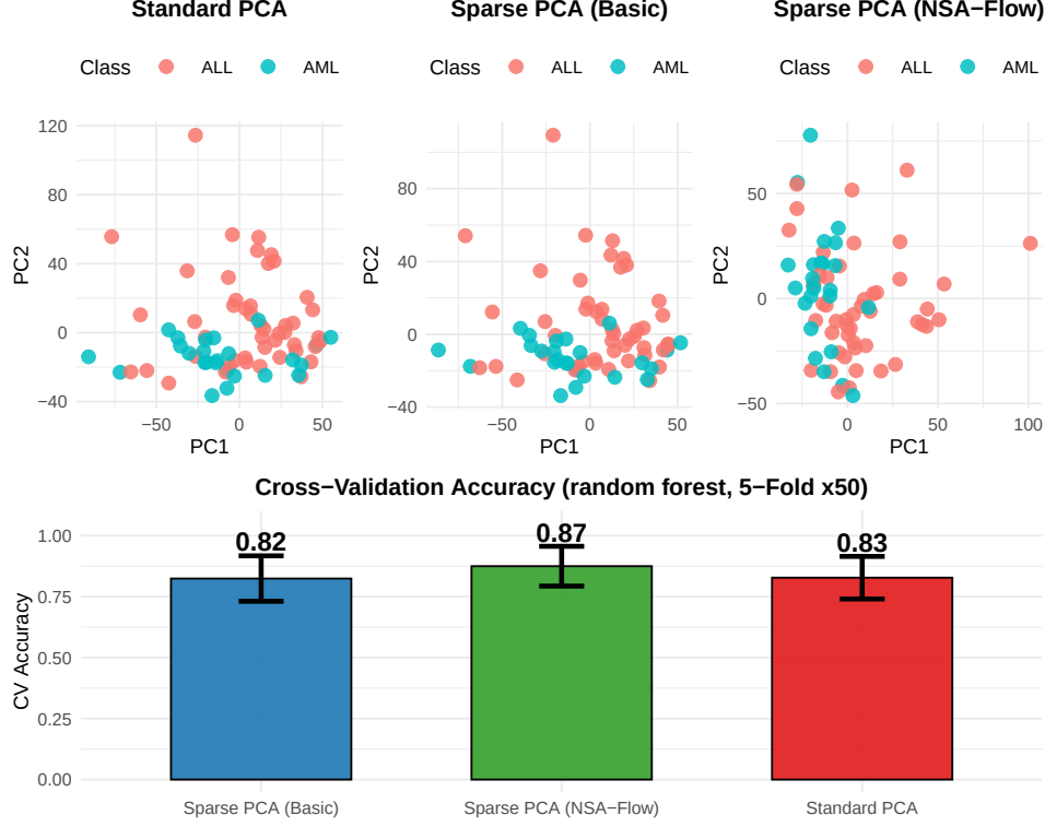
Figure 6: Comparison of PCA Variants on Golub Leukemia Dataset: Core Metrics, 2D Projections, and Classification Performance.
