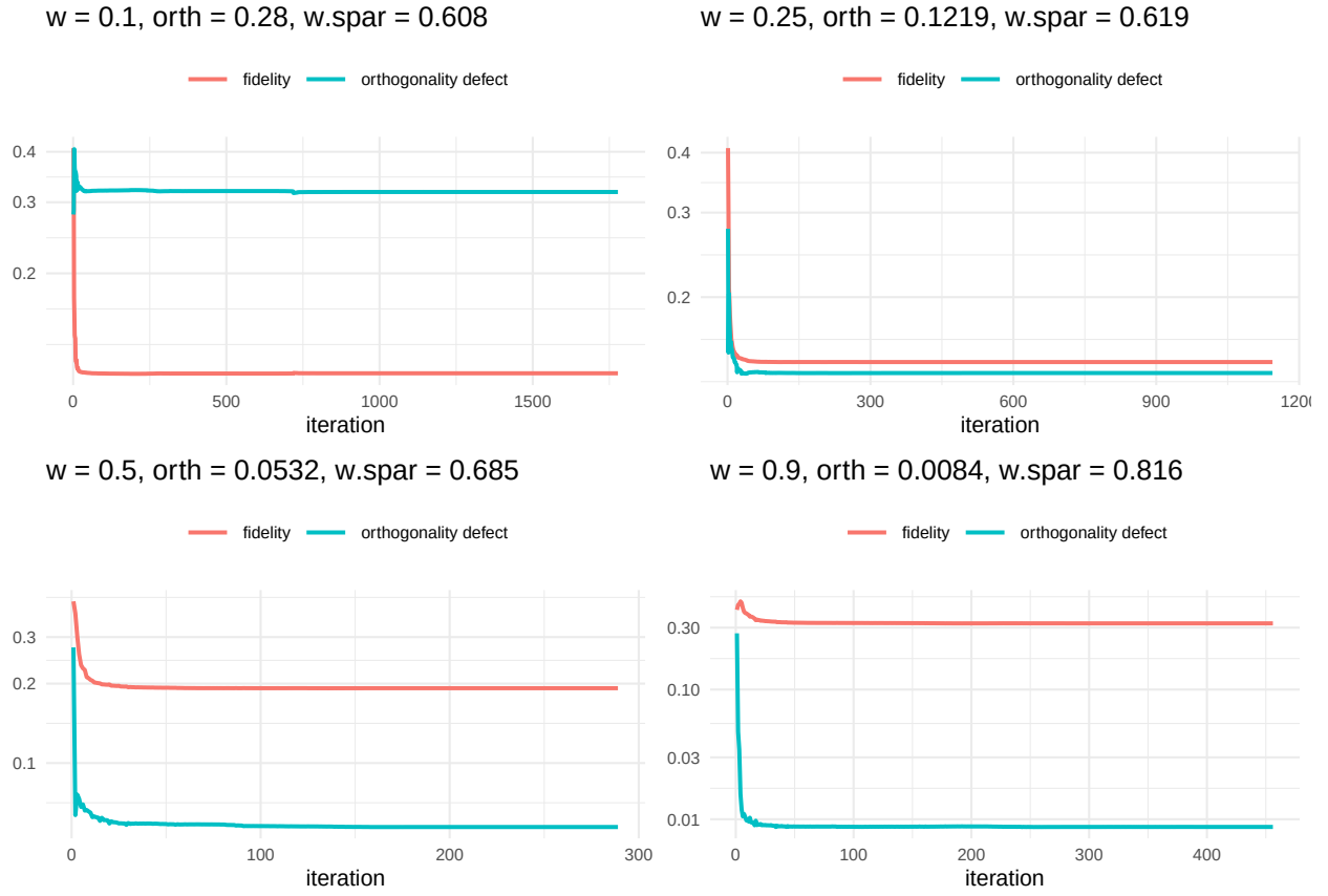
Figure 5: Energy terms against iteration at four values of the orthogonality weight. Fidelity and the orthogonality defect are shown on a log scale; the solver is monotone in the total energy by construction, so both curves are traced from the same accepted steps.
