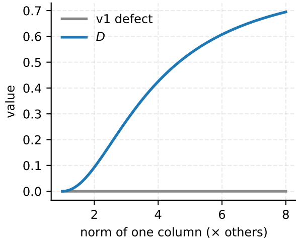
(a) columns stay orthogonal
