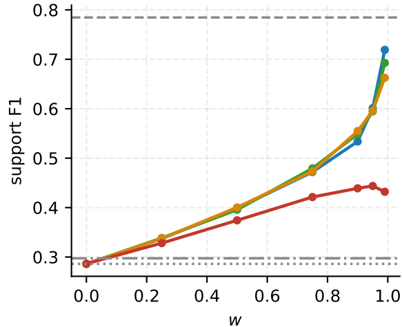
(b) support recovery
