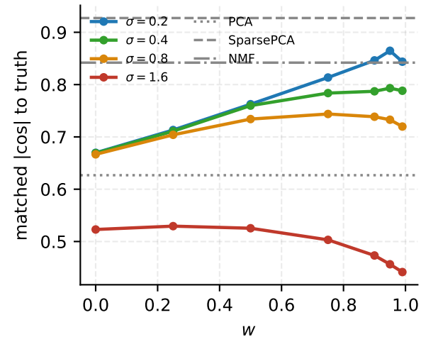
(a) basis recovery
