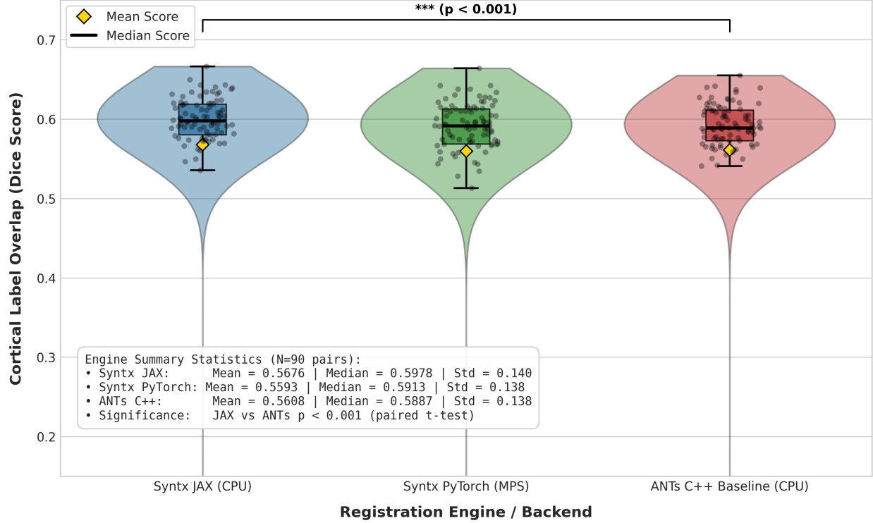
Figure 6: Cortical Dice Distribution Across 90 Mindboggle Benchmark Pairs
