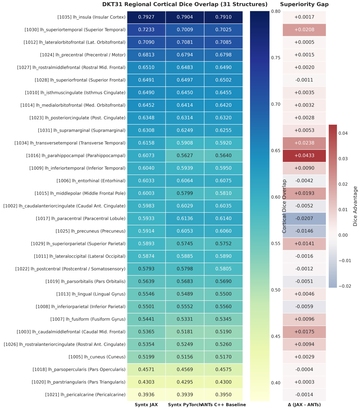
Figure 10: Figure 7: Regional Heatmap of DKT31 Cortical Overlap Across All 31 Individual Structures
