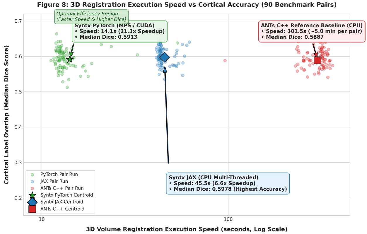
Figure 8: Figure 8: 3D Volume Registration Execution Speed vs Cortical Accuracy
