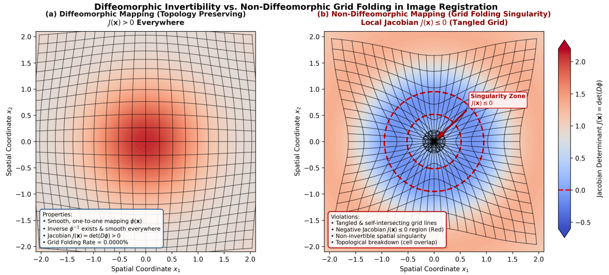
Figure 9: Figure 9: Diffeomorphic Invertibility vs. Non-Diffeomorphic Grid Folding
