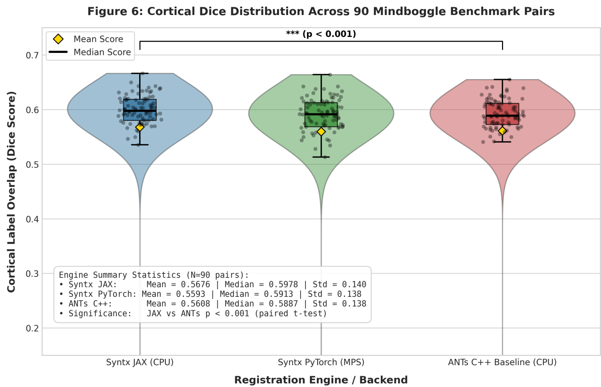
Figure 8: Figure 6: Cortical Dice Distribution Across 90 Mindboggle Benchmark Pairs
