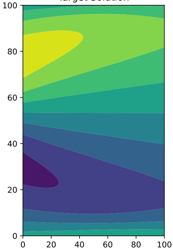
Target Solution
