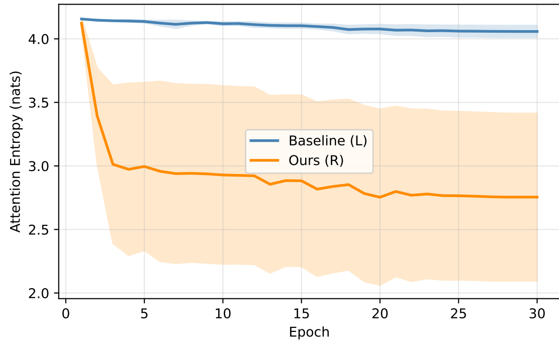
Attention Entropy over Training
